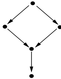
Figure 1: A typical directed acyclic graph (DAG) representing the decomposition of Eq. (2).
