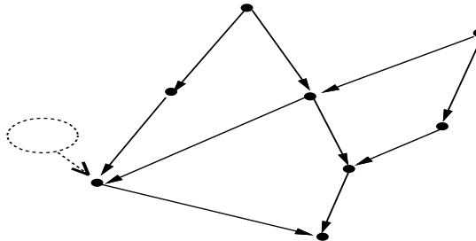
Figure 4: Graphical representation of Rubin’s model, showing the observed response ( Y ) as a function of treatment ( Z ) and causal effect ( \mathbf{r} ) variables.
