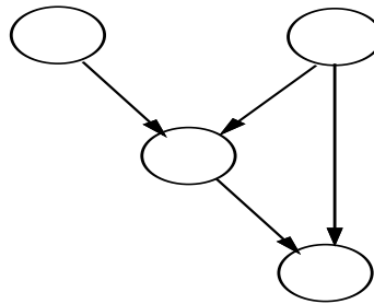
Figure 5: Graphical representation of causal dependencies in a randomized clinical trial with partial compliance.
