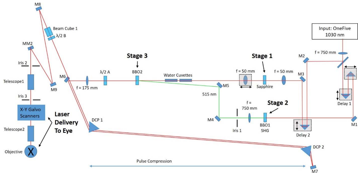
Figure 2. Custom NOPA schematic. Schematic shows the components of the amplified NLO CXL device. The device consists of three main elements: (1) The laser source (OneFive regenerative amplified FS laser) produces 1030 nm amplified FS pulse light. (2) The NOPA consisting of three stages (supercontinuum generation, frequency-doubled pump beam generation, and parametric conversion) is used to alter the wavelength of the input beam to 760 nm. (3) The laser delivery system focuses the resulting 760 nm amplified FS light into the eye. Amplified FS light is directed through the three NOPA stages using a series of mirrors ( M ) and specified focal length lenses ( f ), through a dispersion compensation prism pair (DCP) for pulse compression, and then into the delivery optics.
