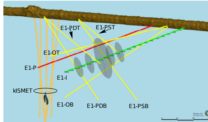
Figure 2: Experiment 1 schematic along the West Drift on the 4850 level of SURF. Green line - stimulation (injection) well (E1-I), red line - production well (E1-P), yellow lines - monitoring wells, and orange lines - kISMET wells. The two monitoring wells originating between E1-I and E1-P – rightmost intersection with the drift (brown) are called OT (“O” for orthogonal to the anticipated hydraulic fracture and “T” for top) and OB (“B” for bottom), the 2 monitoring wells originating midway down-drift are called PST and PSB (“P” for parallel to the anticipated fracture plane, “S” is for shallow), and the most distant monitoring wells are called PDT and PDB where the “D” is for deep. E1-I and E1-P are approximately parallel to S_{hmin} and the gray disks indicate nominal hydraulic fractures.
