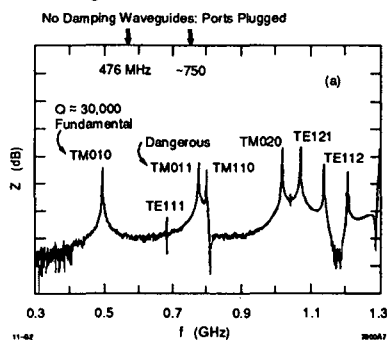
Figure 1. Undamped low power RF cavity impedance.
