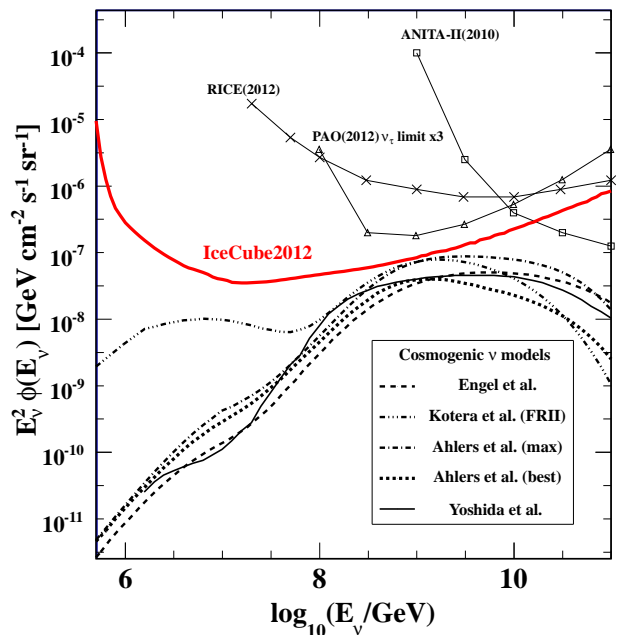
FIG. 9. All flavor neutrino flux differential 90% C.L. upper limit evaluated for each energy with a sliding window of one energy decade from the present IceCube EHE analysis including the IceCube exposure from the previously published result (IC40) [9]. All the systematic errors are included. Various model predictions (assuming primary protons) are shown for comparison; Engel et al. [7], Kotera et al. [17], Ahlers et al. [33], Yoshida et al. [6]. The model-independent differential 90% C.L. upper limits for one energy decade by other experiments are also shown for Auger (PAO) [53], RICE [54], ANITA [14, 15] with appropriate normalization by taking into account the energy bin width and the neutrino flavor. The upper limit for the \nu_\tau flux obtained by Auger is multiplied by three to convert it to an all flavor neutrino flux limit (assuming an equal neutrino flavor ratio).
