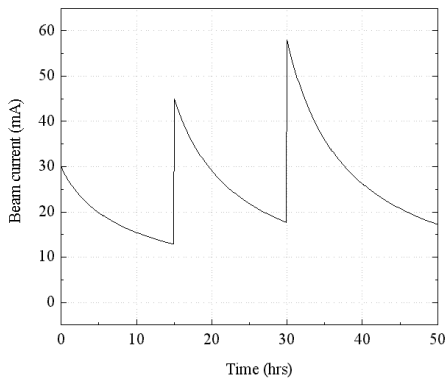
Figure 4. Beam current intensity possible scenario, during the conditioning period in the VLHC, Stage 2, increasing the current from 30 mA to 58 mA (nominal), to avoid large beam scattered power.
