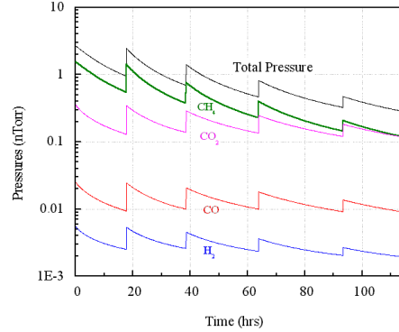
Figure 3. CO scattering equivalent partial pressures and total pressure in the possible conditioning scenario, Stage1.
