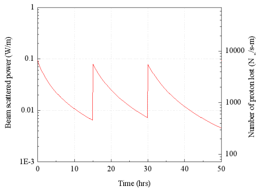
Figure 5. Beam-gas scattered power, and beam-gas scattering proton losses. In Stage 2, the beam is injected increasing the current in three steps to result in a beam scattered power < 0.1 W/m.
