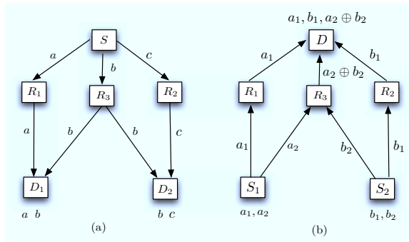
Figure 5.3. (a) is a two-user broadcast network with a common message and (b) is its dual multiple-access network. It is shown that cut-set is achievable using the same linear time invariant code in both cases.
