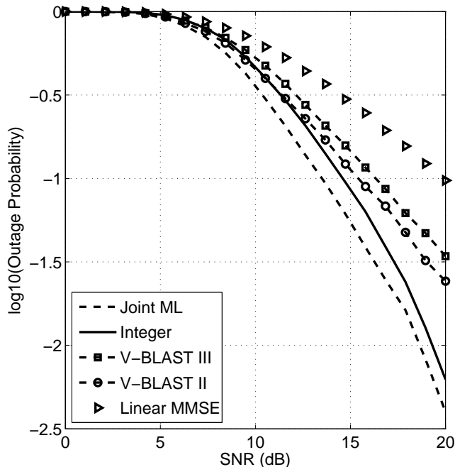
Figure 2.8. Outage probability for the 2 \times 2 complex-valued MIMO channel with Rayleigh fading for a target sum rate of R = 6 .
