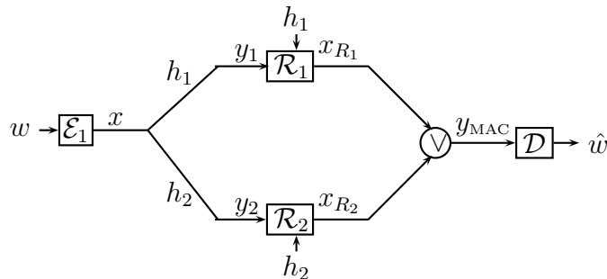
Figure 6.2. The binary network considered in Example 1, with two relays and the binary OR MAC
