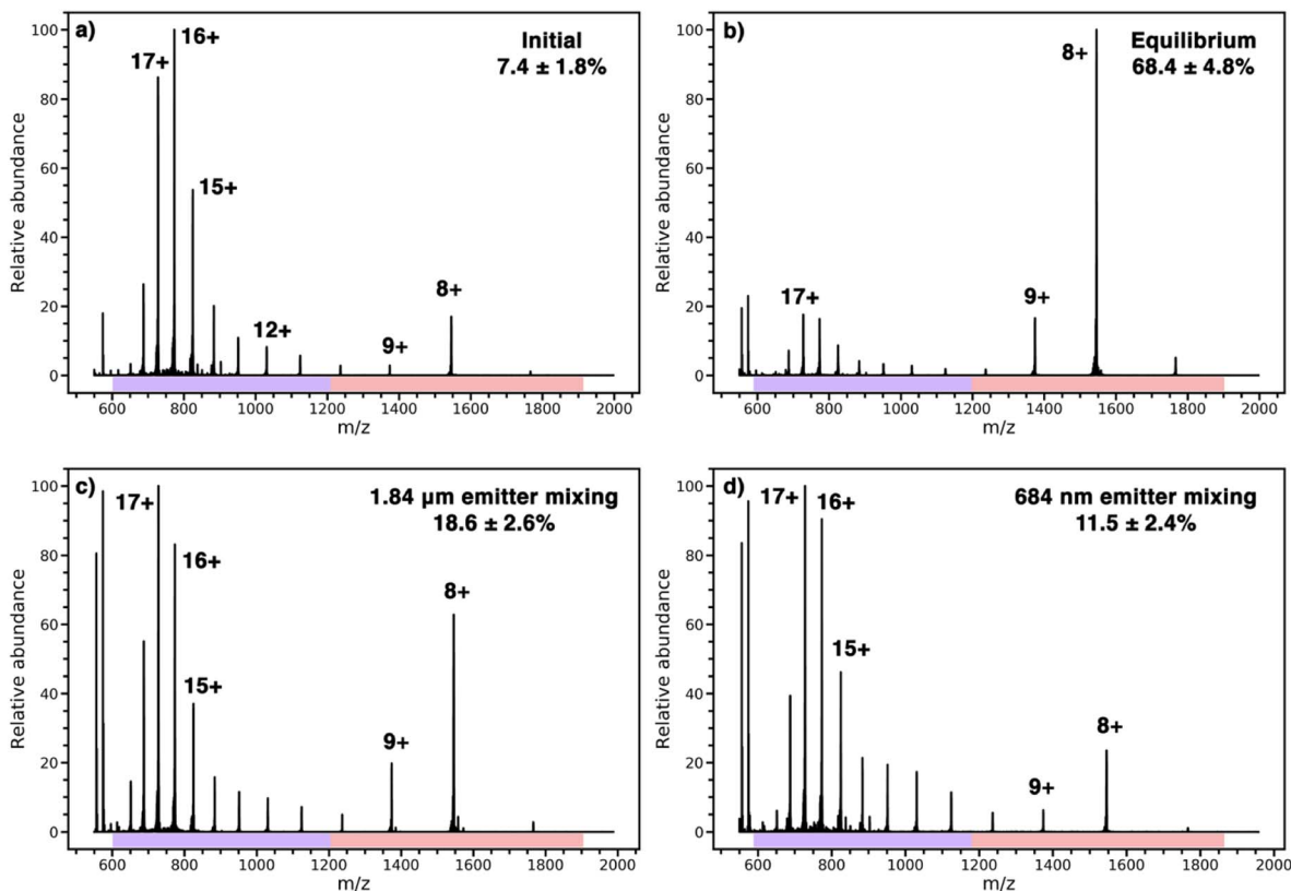
Fig. 3 Representative mass spectra of cytochrome c used to determine the lifetime of nanodrops from the kinetics of protein refolding, (a) an initial solution of cytochrome c with Met-enc ( m/z = 574 ) in water with 1% acetic acid ( \text{pH} = 2.85 ), (b) a 1 : 1 mixture of the solution in (a) with water and Leu-enc ( m/z = 556 ) at equilibrium ( \text{pH} = 3.06 ), (c) theta emitter mixing of solution used in (a) with water containing Leu-enc with 1.84 \mu\text{m} emitters and (d) theta emitter mixing of solution used in (a) and water containing Leu-enc with 684 nm emitters.
