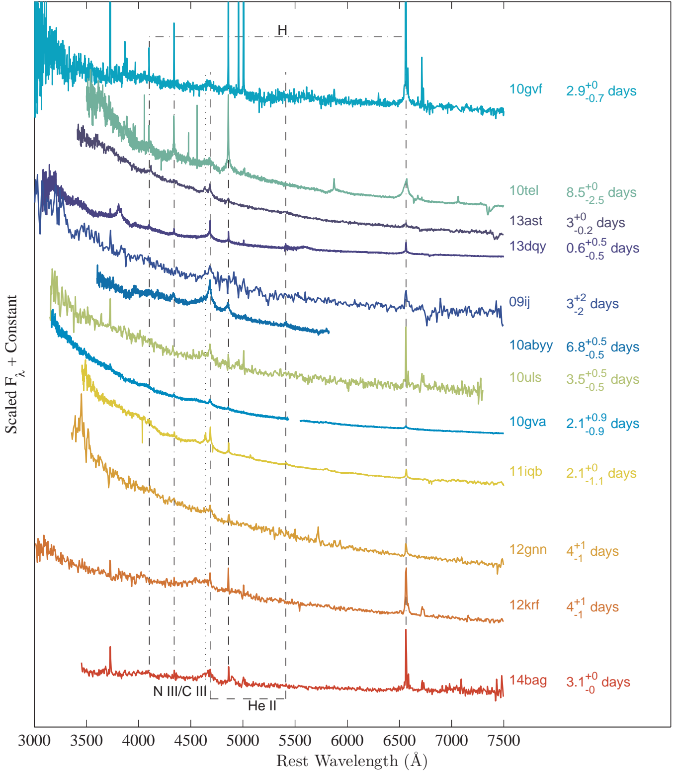
Figure 3. Spectra of our twelve FI events. On the right: an estimate of the age of the SN, with respect to the estimated explosion time (see Appendix A for details).
