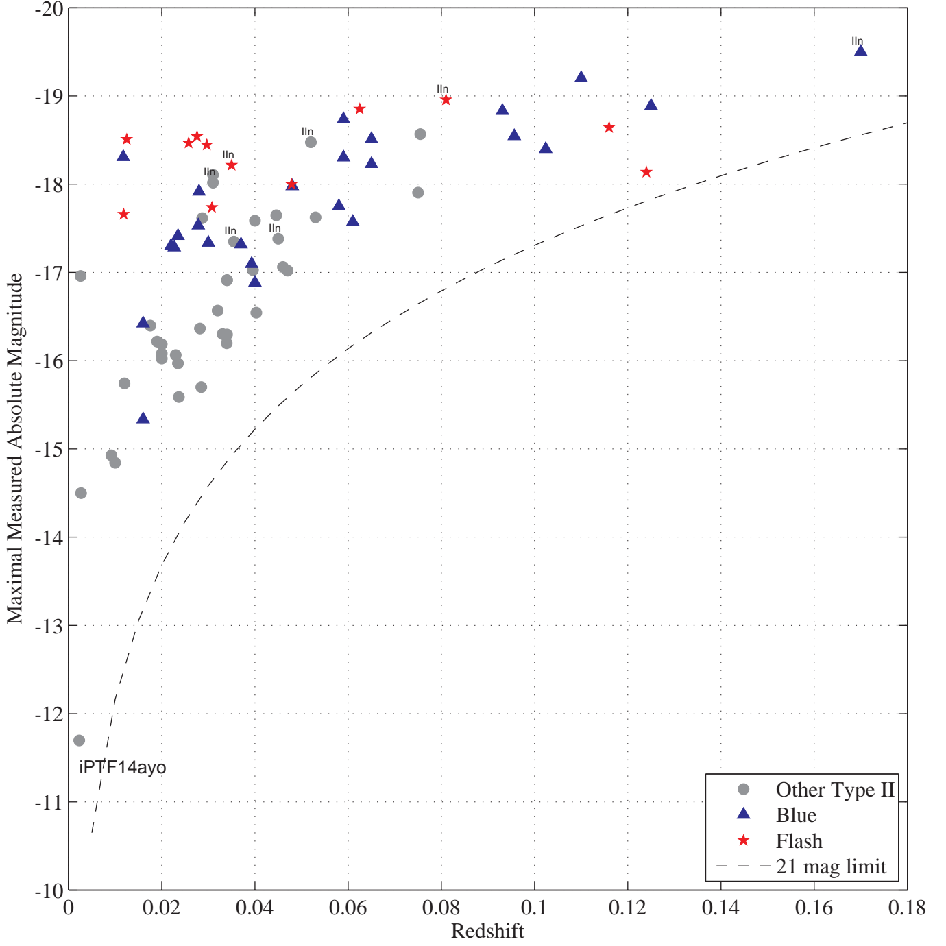
Figure 8. The maximal measured absolute magnitude in the R band (9 events with only early g -band photometry are omitted from this plot; two of these are BF) vs. the redshift. The dashed line corresponds to our average detection limit of R = 21 mag. iPTF14ayo is very faint, probably because of high extinction. FI and BF events dominate the high-luminosity end.
