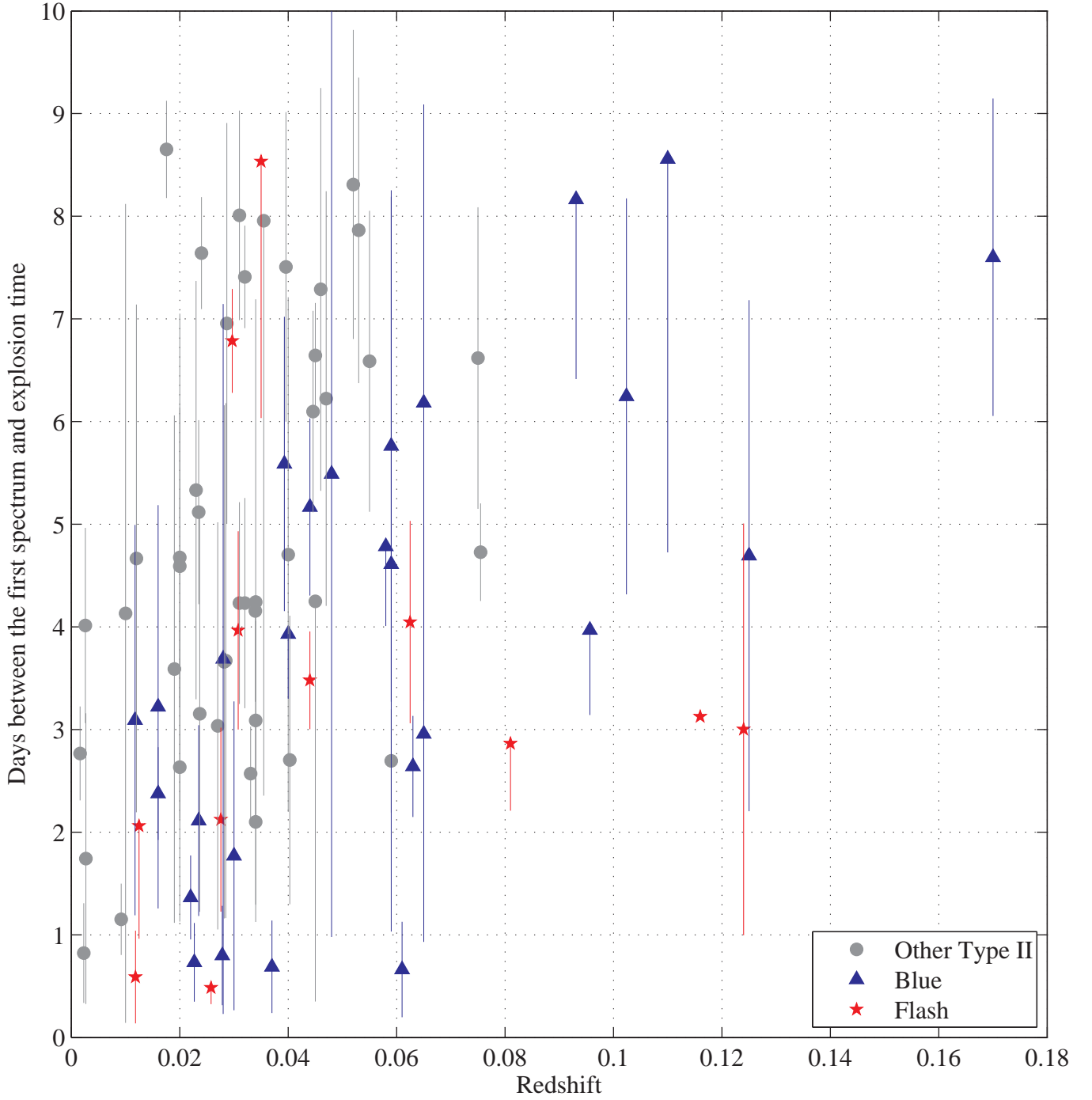
Figure A2. Time between the first spectrum and the estimated explosion time vs. the redshift. The error bars are between the times of the first detection and the pre-explosion limit (which is the same as the estimated explosion time for the SNe with fitted rise time). Note the lack of distant SNe that are not classified as BF or FI events.
