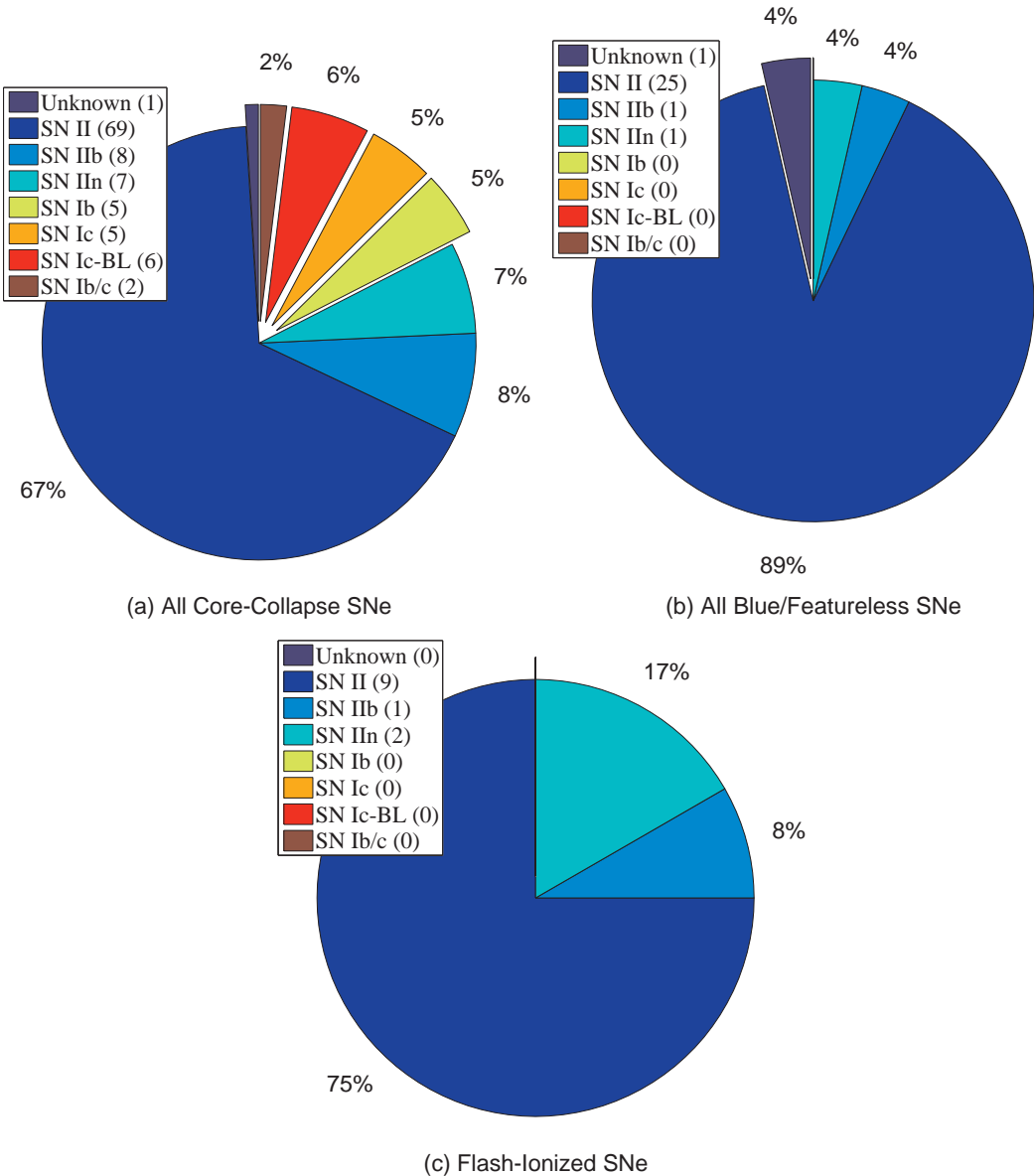
Figure 1. (a) Distribution by type of all 103 CC SNe whose first spectrum was taken < 10 days after the time of the pre-explosion limit. Of these, 84 are SNe II. (b) Type distribution of events with BF first spectra (28 total). (c) Type distribution of FI SNe (12 total). There is only a single, featureless spectrum of the “unknown” SN, not enough for classification.
