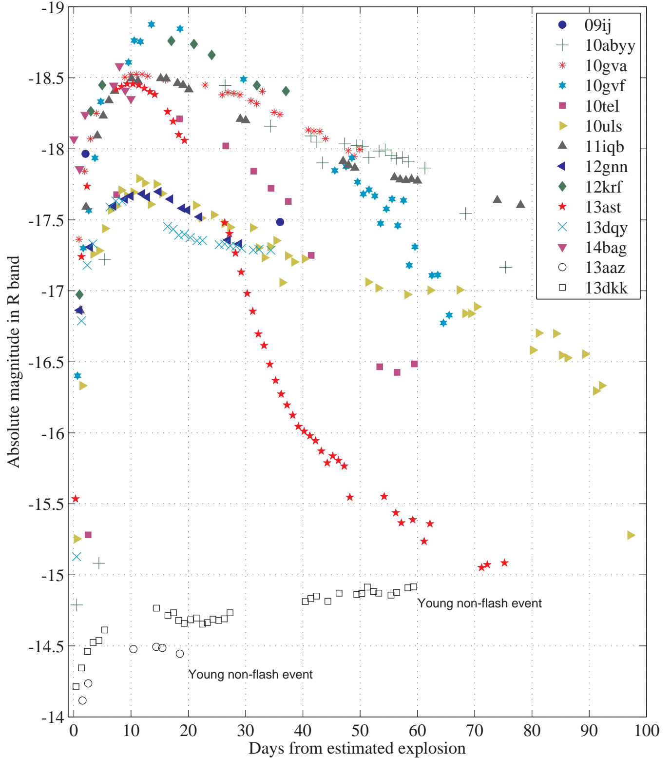
Figure 5. R -band photometry of the twelve flash-spectroscopy events and two (out of the three) events showing neither FI signatures nor a BF continuum in their spectra < 2 days after explosion. The light curve of the highly reddened iPTF14ayo is very faint; it is omitted for clarity. Measurements from the same night have been averaged into a single data point. Error bars are omitted for clarity and are available with the full photometry in the electronic table.
