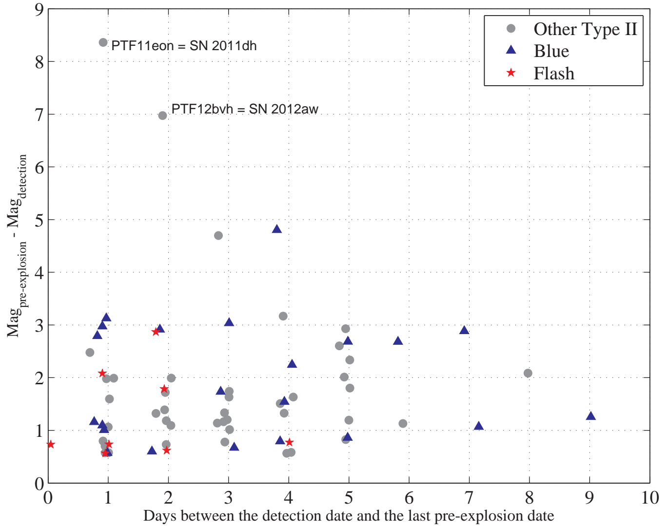
Figure A1. The magnitude difference between the pre-explosion limit and the first detection vs. the difference in days between the first detection and the pre-explosion (last nondetection) limit. All of the events with explosion time estimated by fitting the rise time (rather than using a recent pre-explosion limit) are omitted from this plot. SN 2011dh and SN 2012aw are nearby SNe with very deep nondetection limits, hence the large magnitude difference in a short time.
