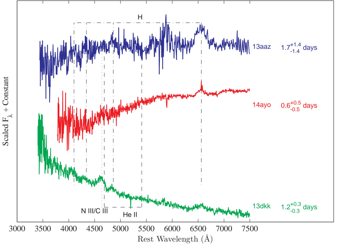
Figure 6. The first spectra of SNe that are < 2 days old and were not classified as FI or BF. At right: the SN age, with respect to the estimated time of explosion (see Appendix A for details).
