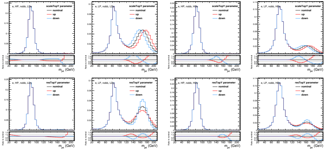
Figure 4.47: Projections of the nominal and alternative shapes of the resonant background onto the m_{\text{jet}} dimension obtained from applying \pm 3\sigma variations of the top peak scale (top) and resolution (bottom) uncertainties for the electron channel in the nobb category. Left to right: HP-LDy, LP-LDy, HP-HDy, LP-HDy.
