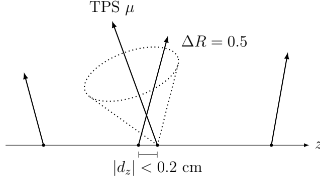
Figure 5.9: Illustration of the track isolation process used by the algorithm. A cone is defined about the origin of the candidate track \text{TPS } \mu , and the algorithm checks if there are any adjacent tracks whose origin is within |d_z| of the \text{TPS } \mu origin, and if the track is within a cone of radius \Delta R centered about \text{TPS } \mu . Tracks for which p_{\text{T,cone}} as defined by equation 5.13 exceeds the threshold set for the algorithm are discarded.
