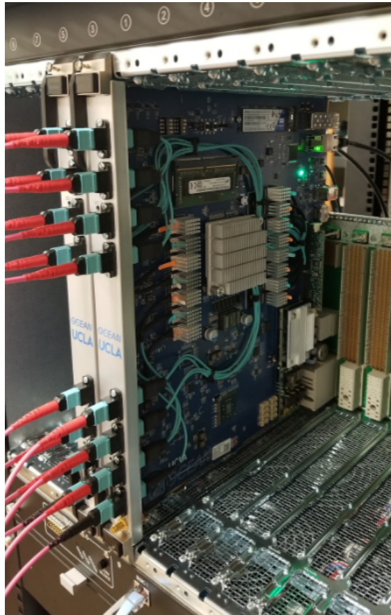
Figure 5.12: Picture of the assembled OCEAN Blade board that will be implemented into the CMS detector hardware. The onboard FPGA will allow for the TPS algorithm to be implemented directly as firmware into the muon trigger in the detector.
