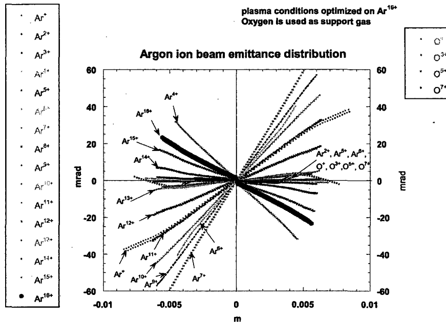
Fig. 6: Different charge states focus differently in the high magnetic field of a superconducting ECR ion source. This leads to typical emittance patterns (at z=15 cm from the outlet aperture), where each charge state is oriented differently in the r - r' phase space.
