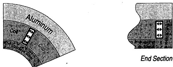
Clamping Principle of the Sextupole "Bladder"
