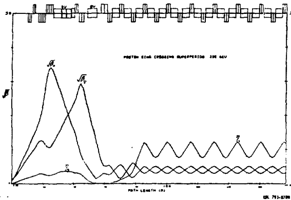
Fig. 2. Proton Ring Crossing Superperiod 300 GeV
