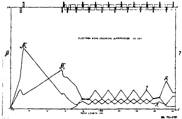
Fig. 3. Electron Ring Crossing Superperiod 15 GeV
