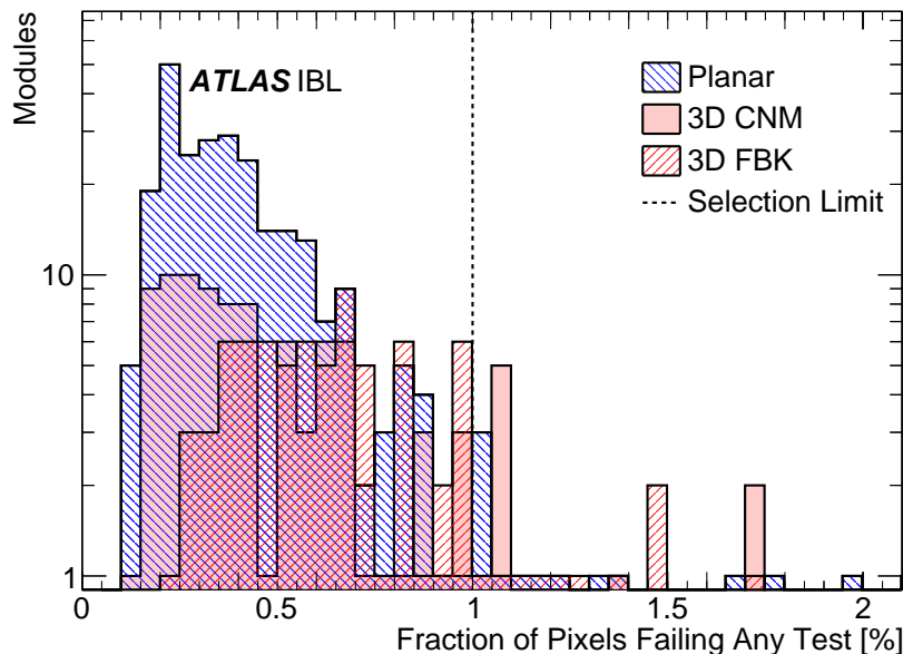
Figure 20. The distribution of the fraction of pixels failing in any test. Only modules otherwise accepted for stave loading are included. The modules are tuned to a 3000 e^- threshold, and 10 ToT counts for a charge injection of 16 ke^- , at a nominal operating temperature of -15^\circ C . A pixel is counted if it fails any one of the tests as described in the text. The selection limit is shown as a vertical line. Overflow entries are not shown.
