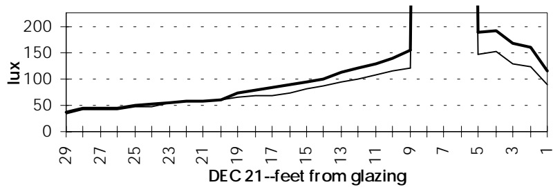
Figure 11. Illuminance distribution at 30 inches above the floor with holographic glazing with 75.6° acceptance and 18° diffraction angles (bold line) versus clear glazing (thin line).
