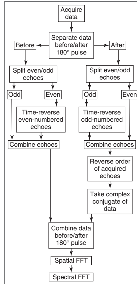
Figure 30.11. Different steps for postprocessing the MEEP-COSI/MEEP-JRESI datasets
