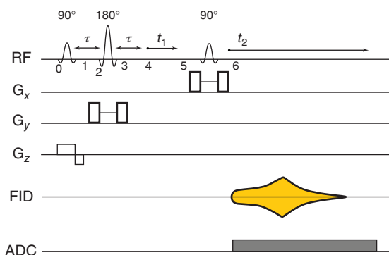
Figure 30.1. A schematic diagram of the 2D L-COSY sequence containing three slice-selective RF pulses ( 90^\circ , 180^\circ , 90^\circ ) for volume localization. The B_0 -crusher gradient pulses were played around the 180^\circ refocusing and the second 90^\circ coherence transfer RF pulses. After the evolution during 2\tau , there is a formation of the Hahn spin echo. Direct acquisition along t_2 and indirect detection along t_1 enable encoding of two spectral dimensions
