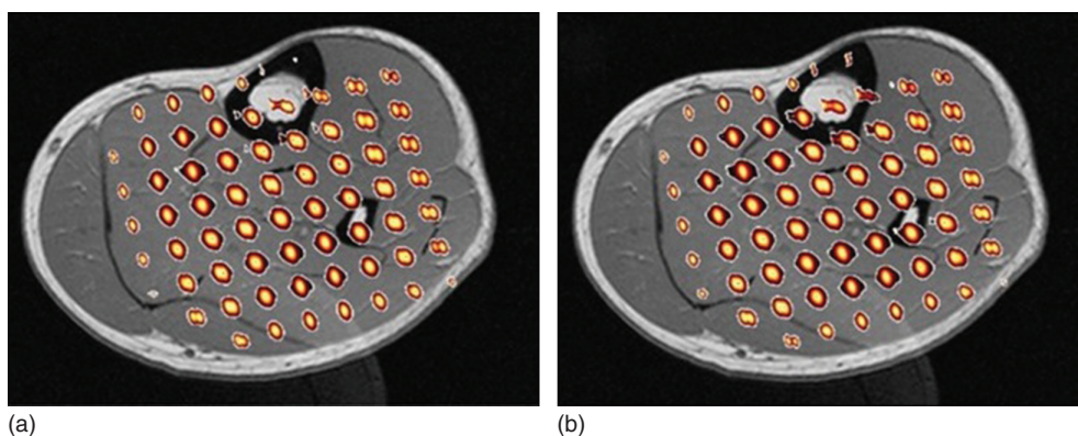
Figure 30.14. Comparison of the performance of the (a) MEEP-COSY and the (b) EP-COSY sequences in the calf of a healthy 28-year-old male volunteer. Spatial projections of the creatine diagonal peak at 3.9 ppm are overlaid on top of T_1 -weighted axial MRI. (Reproduced with permission from Ref. 96. © John Wiley & Sons, Ltd., 2014)
