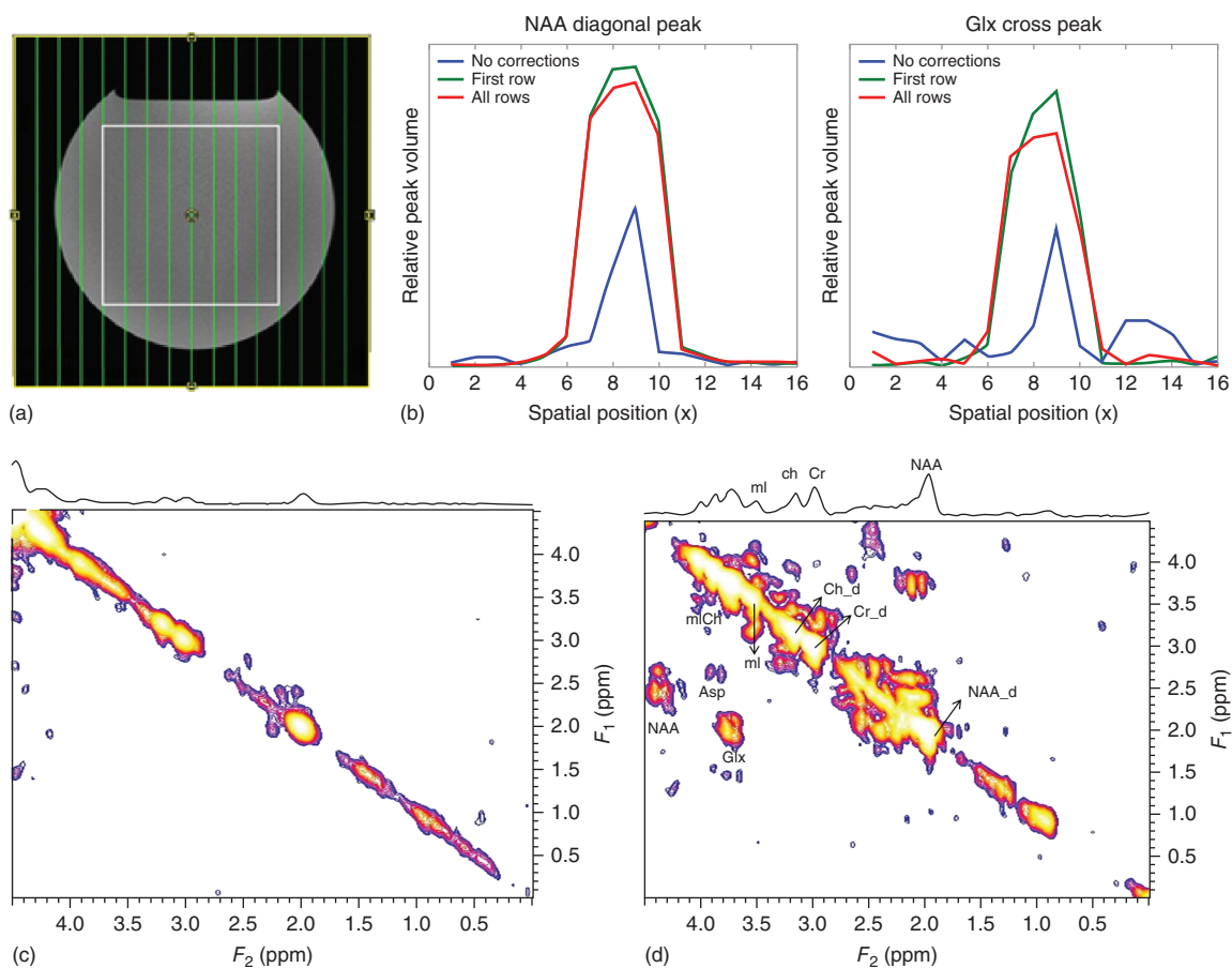
Figure 30.12. (a) Axial MRI of a phantom showing 16 vertical grids for EP-COSI with only one phase-encoding step ( \Delta k_y = 0 ). (b) 1D spatial profiles of the NAA diagonal peak at 2 ppm (left) and glutamate/glutamine (Glx) cross-peaks (right) after postprocessing the EP-COSI data with and without EC corrections. The three colored curves represent three postprocessing methods: no EC corrections are applied (blue), EC corrections are applied only using the first NWS row (green), and EC corrections are applied using all t_1 NWS rows (red). (c) Extracted 2D COSY spectra from one of the columns without and (d) with EC (Klose's) correction
