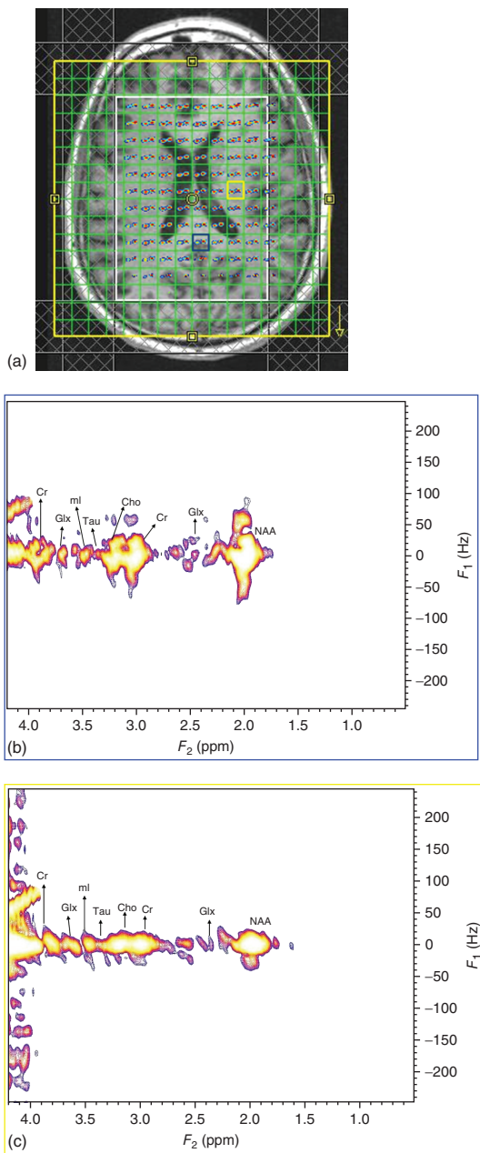
Figure 30.13. (a) Multivoxel spatial distribution of 2D diagonal peaks of Cr and Cho (3.0 and 3.2 ppm) overlaid on a T_1 -weighted axial MRI. The white box indicates PRESS inner-volume localization, with voxels in the mid-occipital and left temporal lobes highlighted in blue and yellow, respectively. (b) Selected 2D J -resolved spectra extracted from the mid-occipital and (c) left temporal voxels
