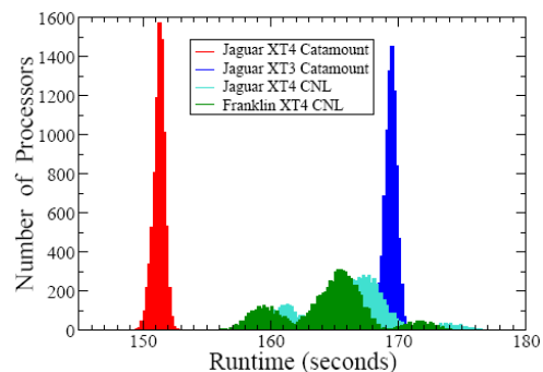
Figure 9. Histogram of run time on Jaguar and Franklin. (Courtesy Van Straalen et al. [10])
