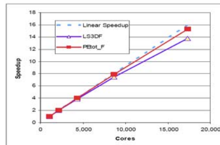
Figure 11. LS3DF and PEtot_F speedup. (Courtesy Wang et al. [14])
