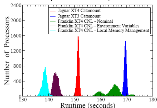
Figure 10. Histogram of run time on Jaguar and Franklin with CLE malloc environment variable setting and with AMR local memory management show a reduced single peak distribution. (Courtesy Van Straalen et al. [10])
