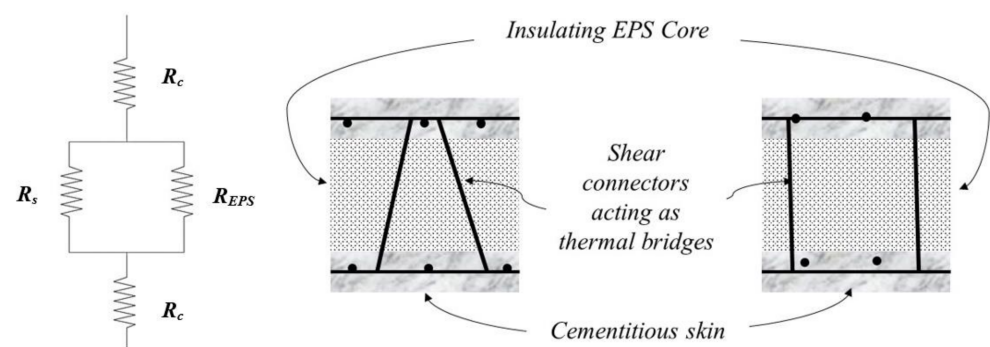
Figure 9. Equivalent thermal circuit for a typical CSP panel.
