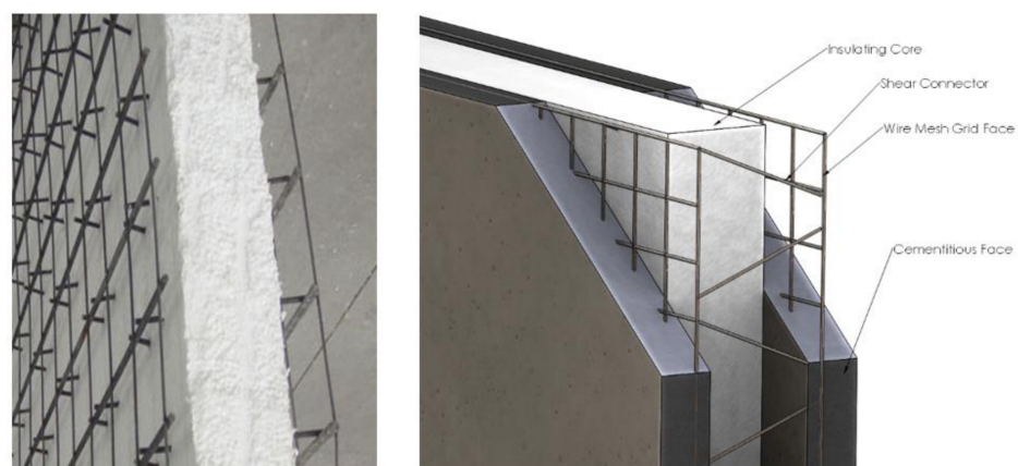
Figure 3. Details of a typical cementitious sandwich panel with individual welded wire shear connectors ( Class I ).
