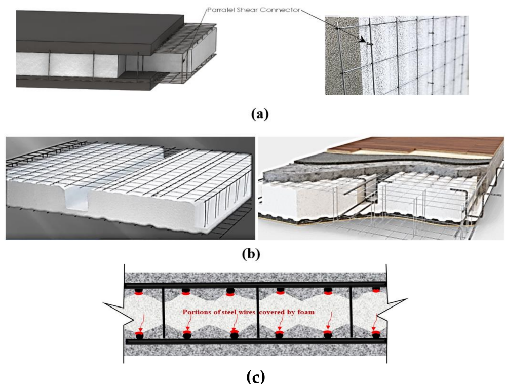
Figure 5. CPS Panels Shear Reinforcements: (a) Panels with parallel wires shear reinforcement ( Class I ), (b) Ribbed floor panels with parallel wires shear reinforcement ( Class II ), (c) Portions of wire surfaces covered by EPS foam.
