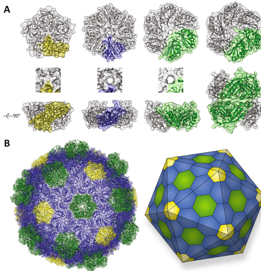
Fig. 1. The BMC structural proteins forming a polyhedral shell. a The four different types of building blocks: BMC-P (pentamer monomer in yellow ); BMC-H hexamer (monomer in blue ); BMC-T S trimer (monomer in green ), and the double stacked BMC-T D hexamer (monomer in each layer in green ). A top view and a side view are shown, as well as a close up of the center for the BMC-P, BMC-H, and BMC-T S . The BMC-T D pore can have an open or closed conformation (closed conformation is shown). The shell proteins have a concave and a convex side, the concave side faces outward (towards the top of the side view), while the convex side faces the BMC lumen (towards the bottom of the side view). b The structure of a BMC shell from Haliangium ochraceum and a schematic of the icosahedral symmetry (BMC-H in blue ; BMC-T S and BMC-T D in green ; BMC-P in yellow )
