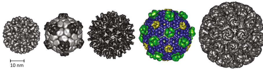
Fig. 6. The size and geometry of virus-like particles used in biomedical engineering in comparison with the BMC shell from Haliangium ochraceum . From left to right: cowpea chlorotic mottle virus (PDB ID 1cwp), cowpea mosaic virus (PDB ID 5fmo), hepatitis B virus capsid (PDB ID 1QGT), Haliangium ochraceum BMC (PDB ID 6MZx), and murine polyomavirus (PDB ID 1sid)
