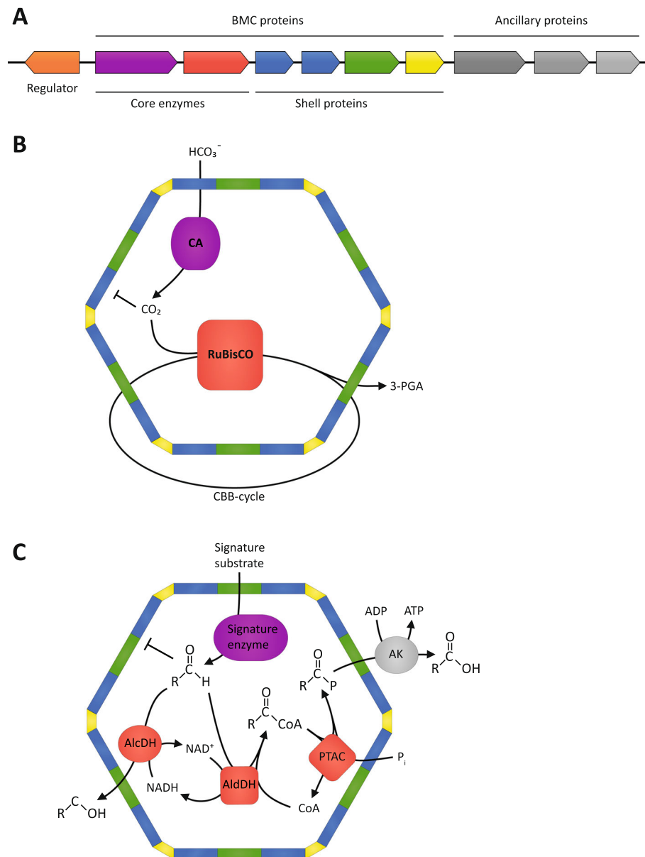
Fig. 2 BMC genetic and metabolic modularity. a Schematic of a BMC gene locus containing a transcriptional regulator (orange) presumably controlling the expression of the BMC operon, the enzymatic core (purple and red), the structural shell proteins (blue, green, and yellow) forming the BMC and the ancillary proteins positioning and metabolically integrating the BMC into the cell (gray). b Schematic function of the carboxysome. The shell acts as a barrier to concentrate the \text{CO}_2 and potentially exclude the competitive inhibitor oxygen within the BMC, enabling RuBisCO to operate more efficiently. 3-PGA 3-phosphoglycerate. c Schematic function of metabolosomes. The toxic aldehyde intermediate is contained and detoxified within the BMC. CoA coenzyme A, \text{P}_i inorganic phosphate
