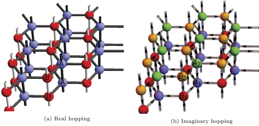
Fig. 6. (a) The tight-binding model on a stacked honeycomb lattice with real-valued nearest-neighbor hopping. Blue/red (A/B) mark the two sub-lattices of the honeycomb lattice respectively. The positive hoppings are drawn in black, while the negative hoppings in white. (b) After the gauge transformation (c_j^{A_1}, c_j^{B_1}, c_j^{A_2}, c_j^{B_2}) \rightarrow (c_j^{A_1}, ic_j^{B_1}, ic_j^{A_2}, c_j^{B_2}) , a unit cell contains four sites. This is marked by blue/red/green/orange and labeled as A_1/B_1/A_2/B_2 respectively. The hoppings become purely imaginary. The arrows point in the direction where the hopping is +it . The tight-binding Hamiltonian in panel (b) has charge-SU(2) symmetry.
