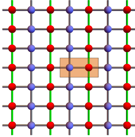
Fig. 2. The \pi -flux mean-field theory. Here the black bonds represent hopping amplitude i\chi in the positive x- or y-direction and the green bonds represent -i\chi . The unit cell is enclosed by the orange rectangle.
