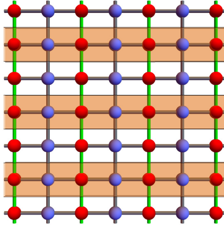
Fig. 3. Translation by one lattice constant in the x-direction compounded with the gauge transformation which multiplies the fermion operators on sites in the orange rows by -1 leaves the mean-field Hamiltonian invariant.
