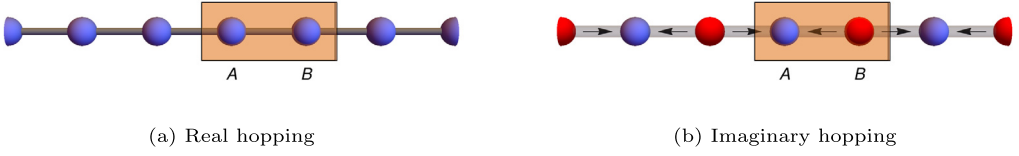
Fig. 4. (a) The usual 1D nearest neighbor tight-binding with real hopping. (b) Upon the gauge transformation (c_j^A, c_j^B) \rightarrow (c_j^A, i c_j^B) , hoppings become purely imaginary with alternating sign. The arrows point in the direction where the hopping is +it . The hopping Hamiltonian in panel (b) is charge-SU(2) invariant.
