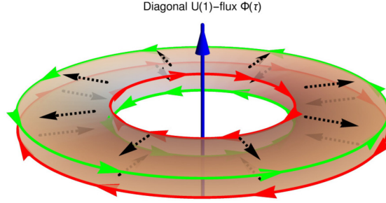
Fig. 1. Two layers of annulus shape Chern insulators with \sigma_{xy} = \pm 1 stacked together. The outer edge harbors the 1D n = 1 non-chiral massless fermion modes. The green and red arrows represent the opposite chiralities. When a time-dependent diagonal U(1) flux pierces the inner hole, the induced electric field in the azimuthal direction causes a Hall current (dashed arrows) flowing from inner to outer boundary in the top layer and from outer to inner boundary in the bottom layer. As the result, the chiral current J_+ - J_- is not conserved viewed from the outer edge alone. This system is realized as the “spin Hall insulator” experimentally. (For interpretation of the colors in the figure(s), the reader is referred to the web version of this article.)
