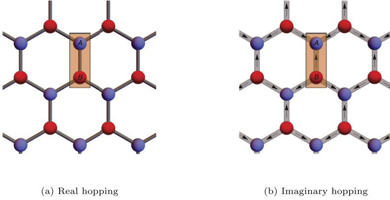
Fig. 5. (a) The usual nearest neighbor tight-binding model on the honeycomb lattice with real hopping. (b) Upon the gauge transformation (c_j^A, c_j^B) \rightarrow (c_j^A, i c_j^B) , hoppings become purely imaginary with alternating sign. The arrows point in the direction where the hopping is +it . The tight-binding Hamiltonian in panel (b) is charge-SU(2) invariant.
