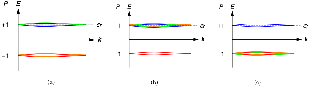
Fig. 8. A caricature of the possible flavor polarization at (a) \nu = 2 and (b) \nu = 1 and (c) \nu = 3 . Note that as long as the Fermi level intersects bands with the right degeneracy, the bands below the Fermi energy can overlap without changing the filling factor. For \nu = -2, -1, -3 we simply reflect the figures with respect to the x -axis.
