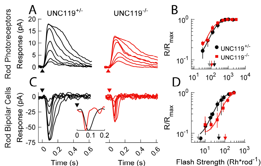
Figure 4. Current responses of rods and rod bipolar cells after exposure to bright light. Mice were exposed to bright bleaching light to translocate transducin to the rod inner segments and were then placed in darkness for 30 min to allow recovery of about 65% of the visual pigment. (A) Representative flash response families from littermate UNC119 +/− (black) and UNC119 −/− (red) rods in the dark-adapted retina. Timing of 20 ms flashes indicated by arrowheads. Intensities were 32, 64, 130, 260, 420, 600, 900, and 1900 Rh* rod −1 for UNC119 +/− ; and 32, 64, 130, 260, 420, 600, 900, 1900, and 2900 Rh* rod −1 for UNC119 −/− . (B) Response–intensity relationships for dark-adapted rods from UNC119 +/− (black) and UNC119 −/− (red) mice, plotted as in Figure 3B. Downward arrows give best-fitting values of I 1/2 from Eqn. (1). Included for comparison is the value of I 1/2 for WT rods (gray) provided in Majumder et al. [16]. (C) Representative flash response families from UNC119 +/− and UNC119 −/− rod bipolar cells. Flash intensities for UNC119 +/− were 5.5, 11, 22, 44, 72, 100, and 150 Rh* rod −1 for UNC119 +/− and 10, 20, 41, 82, 140, 190, and 290 Rh* rod −1 for UNC119 −/− . Inset: representative response waveforms for UNC119 +/− (black) and UNC119 −/− (red) rod bipolar cells to dim flashes. (D) Response–intensity relationships for light-adapted bipolar cells as in (C) from UNC119 +/− (black) and UNC119 −/− (red) mice. Downward arrows give best-fitting values of I 1/2 for rod bipolar cells in UNC119 +/− (black) and UNC119 −/− (red) mice, with comparison to the value in WT rods (gray) from Majumder et al. [16].
