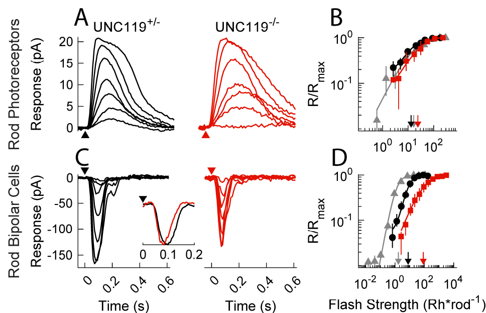
Figure 3. Photocurrent responses of rods and rod bipolar cells in the dark-adapted retina. (A) Representative flash response families from littermate control UNC119 +/− (black) and UNC119 −/− (red) rods in the dark-adapted retina. Timing of 20 ms flashes indicated by arrowheads. Intensities were 2.6, 5.2, 10, 21, 42, 83, and 170 Rh* rod −1 for UNC119 +/− rods and 3.9, 7.8, 16, 31, 62, 120, and 250 Rh* rod −1 for UNC119 −/− rods. (B) Response–intensity relationships for dark-adapted rods from WT (gray), UNC119 +/− (black) and UNC119 −/− (red) mice. Normalized response was plotted against calculated flash intensity in Rh* rod −1 . Sensitivity was estimated from the half-maximal flash strength of the Hill curve (Materials and Methods, Eqn. 1) as indicated by downward arrows. (C) Representative flash response families from UNC119 +/− and UNC119 −/− rod bipolar cells. Intensities of UNC119 +/− were 0.66, 1.3, 2.7, 5.3, 11, 21, and 42 Rh* rod −1 and for UNC119 −/− were 12, 23, 47, 93, 190, 370, and 750 Rh* rod −1 . Inset: representative response waveforms to dim flashes for UNC119 +/− (black) and UNC119 −/− (red) rod bipolar cells. (D) Response–intensity relationships as in (B) but from bipolar cells of WT (gray), UNC119 +/− (black) and UNC119 −/− (red) mice with half-maximal flash strength of the Hill curve indicated by downward arrows.
