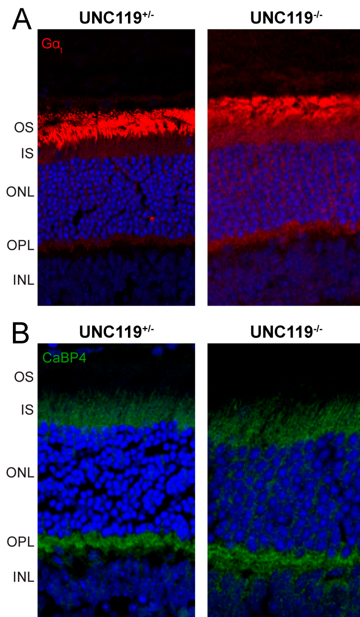
Figure 2. Localization of transducin (A) and CaBP4 (B) in dark-adapted retinas of UNC119 +/- and UNC119 -/- mice with immunofluorescence with anti-Gα t and CaBP4 antibodies. INL, inner nuclear layer; IPL, inner plexiform layer; IS, rod inner segments; ONL, outer nuclear layer; OPL, outer plexiform layer; and OS, rod outer segments. Magnification: 40×.
