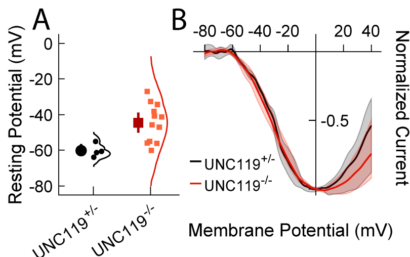
Figure 6. (A) Resting membrane potentials of rod bipolar cells from UNC119 +/- (left) and UNC119 -/- (right) mice. Large symbols give mean with 95% confidence intervals. Smaller symbols are individual measurements clustered as shown. (B) Ca 2+ currents recorded from UNC119 +/- (black) and UNC119 -/- (red) rods with voltage ramps (see Materials and Methods). Shaded regions are 95% confidence limits.
