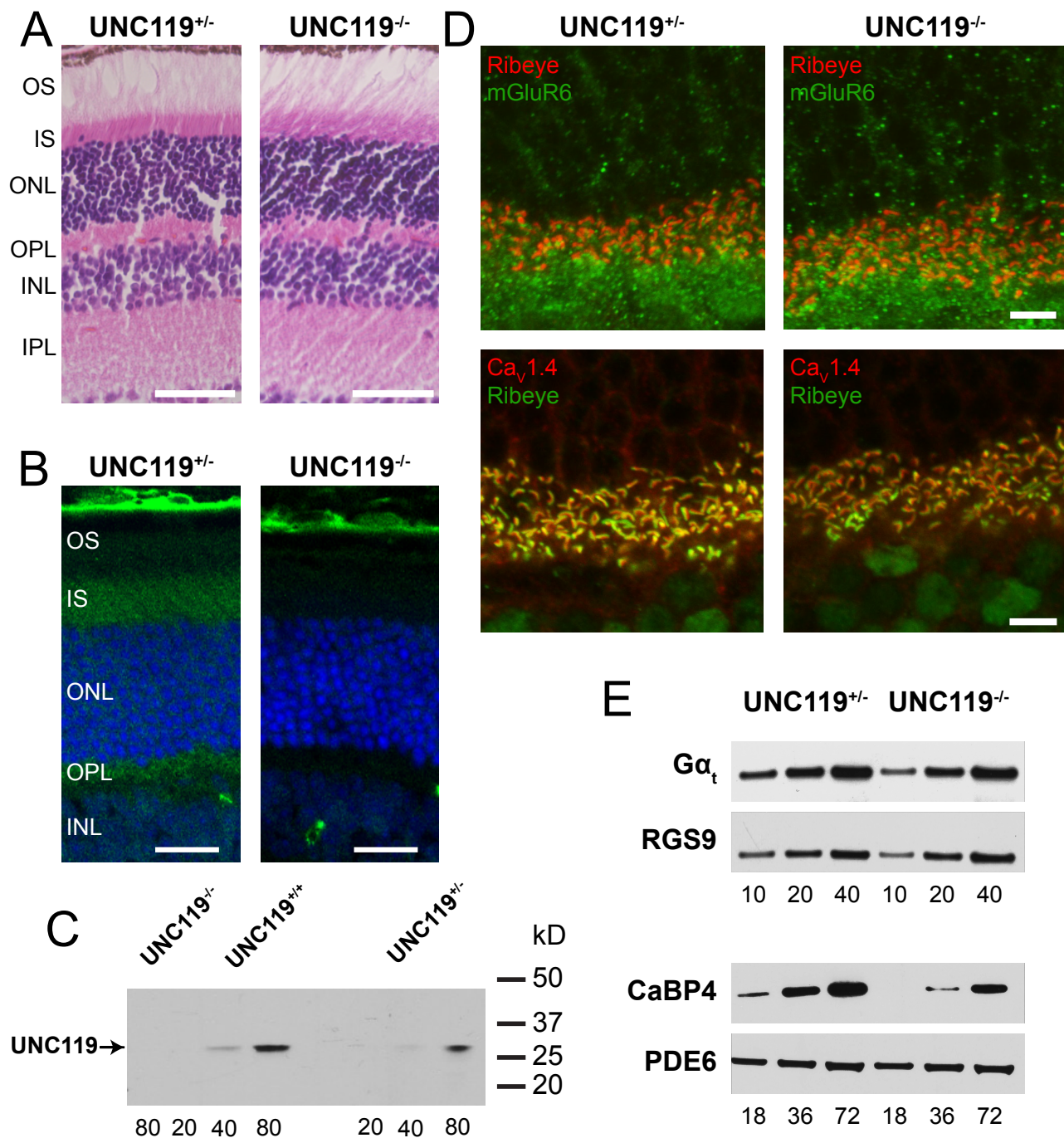
Figure 1. Characterization of UNC119 knockout mouse retinas. (A) Retinal morphology of UNC119 +/- (control) and UNC119 -/- mice. INL, inner nuclear layer; IPL, inner plexiform layer; IS, rod inner segments; ONL, outer nuclear layer; OPL, outer plexiform layer; and OS, rod outer segments. (B) Localization of UNC119 in dark-adapted retinas. Retinas have been stained with a monoclonal antibody for UNC119 [14], followed by goat anti-rabbit AlexaFluor 546. (C) Western blot with antibody for UNC119. Numbers on right are molecular weights in kD determined from BSA and carbonic anhydrase standards. Numbers below lanes are µg soluble retinal protein. (D) Localization of rod-to-rod-bipolar-cell synaptic proteins Ribeye, mGluR6, and Ca v 1.4 in UNC119 +/- and UNC119 -/- mice from immunofluorescence. (E) Immunoblot analysis of expression of various photoreceptor transduction proteins, such as Gα t , RGS9, CaBP4, and PDE6 in UNC119 +/- and UNC119 -/- mice. Numbers below lanes are µg soluble retinal protein. Magnification: 40×.
