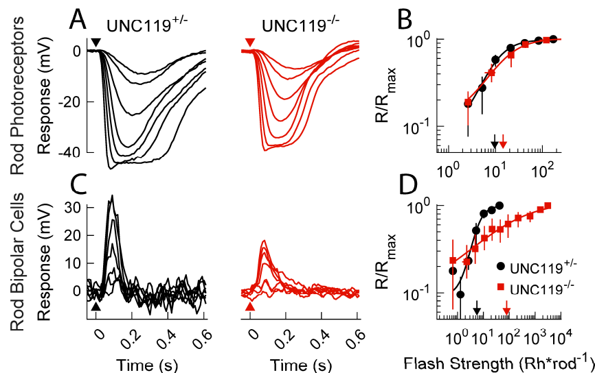
Figure 5. Photovoltage responses of rods and rod bipolar cells in the dark-adapted retina. (A) Representative flash response families from heterozygous littermate controls ( \text{UNC119}^{+/-} ) and \text{UNC119} knockout ( \text{UNC119}^{-/-} ) rods in the dark-adapted retina. Timing of 20 ms flashes indicated by arrow-heads. Intensities were 2.6, 5.2, 10, 21, 42, 83, and 170 \text{Rh}^* \text{rod}^{-1} for both \text{UNC119}^{+/-} and \text{UNC119}^{-/-} . (B) Response–intensity relationships for dark-adapted rods from \text{UNC119}^{+/-} (black) and \text{UNC119}^{-/-} (red) mice. Sensitivity ( I_{1/2} ) is indicated by downward arrows. (C) Representative flash response families from \text{UNC119}^{+/-} and \text{UNC119}^{-/-} rod bipolar cells. Intensities of 20 ms flashes were 0.66, 1.3, 2.7, 5.3, 11, 21, and 42 \text{Rh}^* \text{rod}^{-1} for \text{UNC119}^{+/-} (black) and 49, 97, 190, 390, 780, 1600, and 3100 \text{Rh}^* \text{rod}^{-1} for \text{UNC119}^{-/-} rod bipolar cells (D) Response–intensity relationships as in (B) for dark-adapted rod bipolar cells from \text{UNC119}^{+/-} (black) and \text{UNC119}^{-/-} (red) mice.
