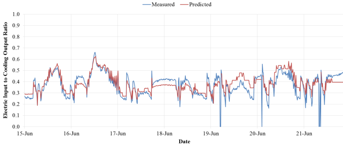
Figure 12: Validation of calibrated chiller model curve – Electric input to cooling output ratio
