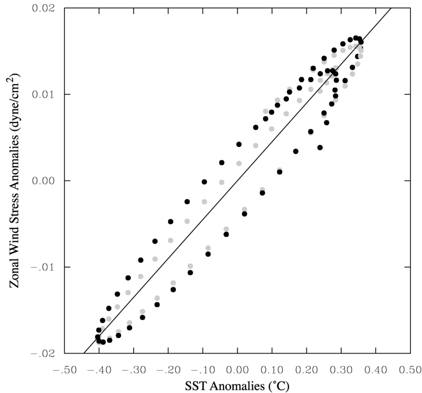
FIG. 11. Scatterplot for zonal wind stress ( [\tau] ) and SST ( T_E ) anomalies of the CGCM ENSO cycle. Dark points are for zonal wind stress ( [\tau] ) anomalies estimated by the modified atmospheric model of Eq. (25) using the simulated SST anomalies ( T_E ). Gray points and the line are from those of Fig. 6.
