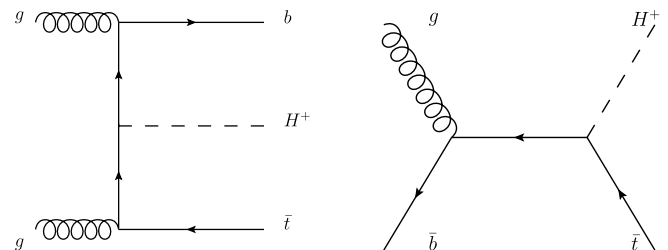
Fig. 1. Leading-order Feynman diagrams for the production of a charged Higgs boson with a mass m_{H^\pm} > m_{\text{top}} , in association with a single top quark (left in the 4FS, and right in the 5FS).
