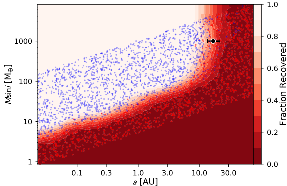
Figure 4. Sensitivity of the HR 5183 RV time series to injected planetary signals as a function of semimajor axis ( a ) and minimum mass ( M \sin i ). Each point corresponds to an injected radial velocity signal. Blue dots were detected, while red dots were not. The solid-color background shows the fraction of signals that were recovered, corresponding to the probability of detection. The parameters of HR 5183 b are shown as a black point with error bars (the uncertainty on M \sin i is too small see). Our data are sensitive to less massive, shorter-period planets out to the orbit of HR 5183 b.
