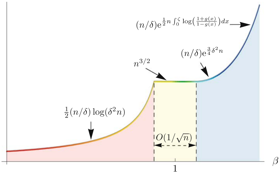
Fig. 1. Illustration of the mixing time evolution as a function of the inverse-temperature \beta , with a scaling window of order 1/\sqrt{n} around the critical point. We write \delta = |\beta - 1| and let \zeta be the unique positive root of g(x) := \frac{\tanh(\beta x) - x}{1 - x \tanh(\beta x)} . Cutoff only occurs at high temperature
