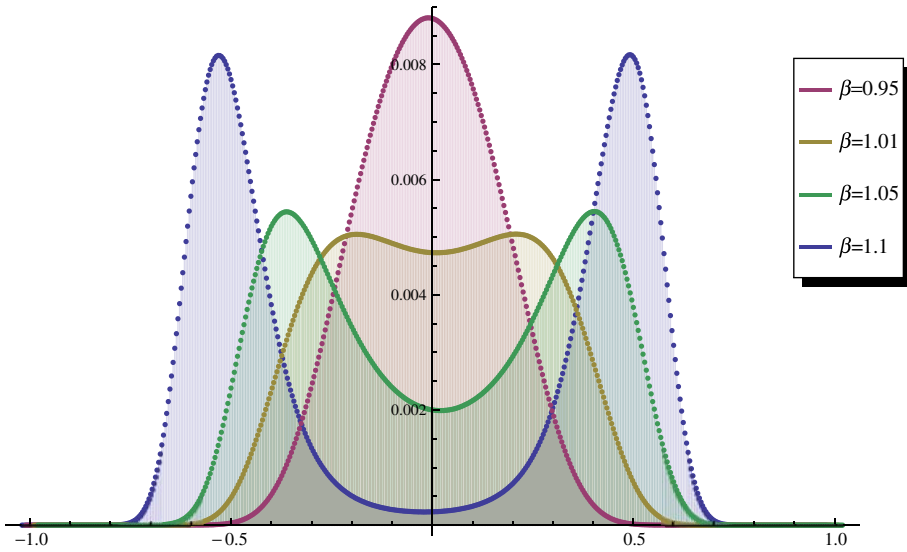
Fig. 2. The stationary distribution of the normalized magnetization chain (average of all spins) for the dynamics on n = 500 vertices. The center of mass at high temperatures (see \beta = 0.95 ) is at 0. Low temperatures feature two centers of mass at \pm\zeta (where \zeta is the unique positive solution of \tanh(\beta x) = x ), leading to the exponential mixing time
