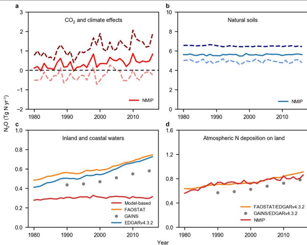
Extended Data Fig. 6 | Global N 2 O emissions from natural soils, inland and coastal waters and due to change in climate, atmospheric CO 2 and nitrogen deposition. a, Changes in global soil N 2 O fluxes due to changing CO 2 and climate. b, Global natural soil N 2 O emissions without consideration of land use change (for example, deforestation) and without consideration of indirect anthropogenic effects via global change (that is, climate, increased CO 2 and atmospheric nitrogen deposition). The estimates are based on NMIP estimates during 1980–2016 including six process-based land biosphere models. Here, we also subtracted the difference between including and not including emissions from secondary forests (that grow back after pasture or cropland abandonment) as part of natural soil emissions based on NMIP estimates.
