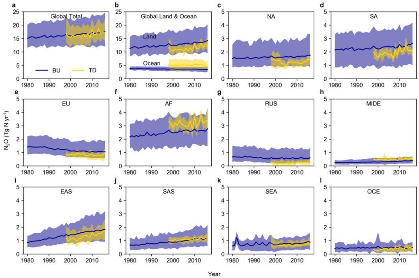
Extended Data Fig. 3 | Comparison of annual total N 2 O emissions at global and regional scales estimated by bottom-up and top-down approaches. The blue lines represent the mean N 2 O emission from bottom-up methods and
