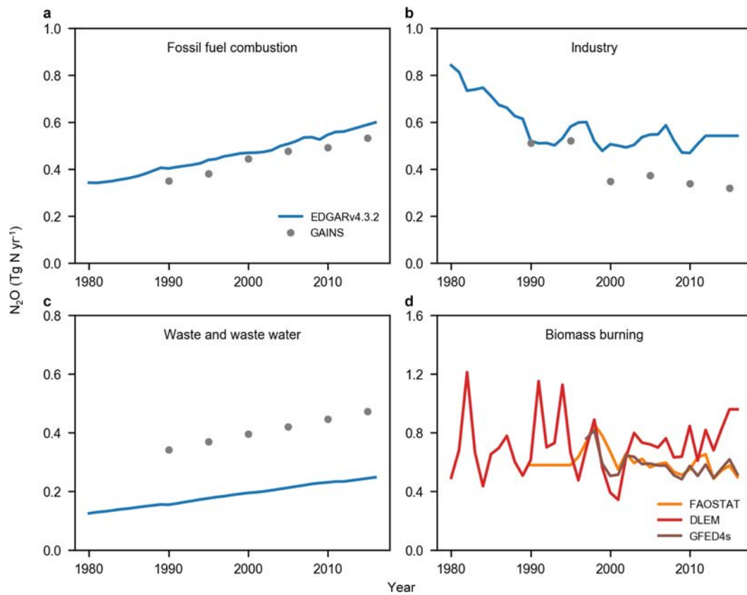
Extended Data Fig. 5 | Global N 2 O emission from other direct anthropogenic sources. a , Emission from fossil fuel combustion based on EDGAR v4.3.2 and GAINS estimates. b , Emission from industry based on EDGAR
