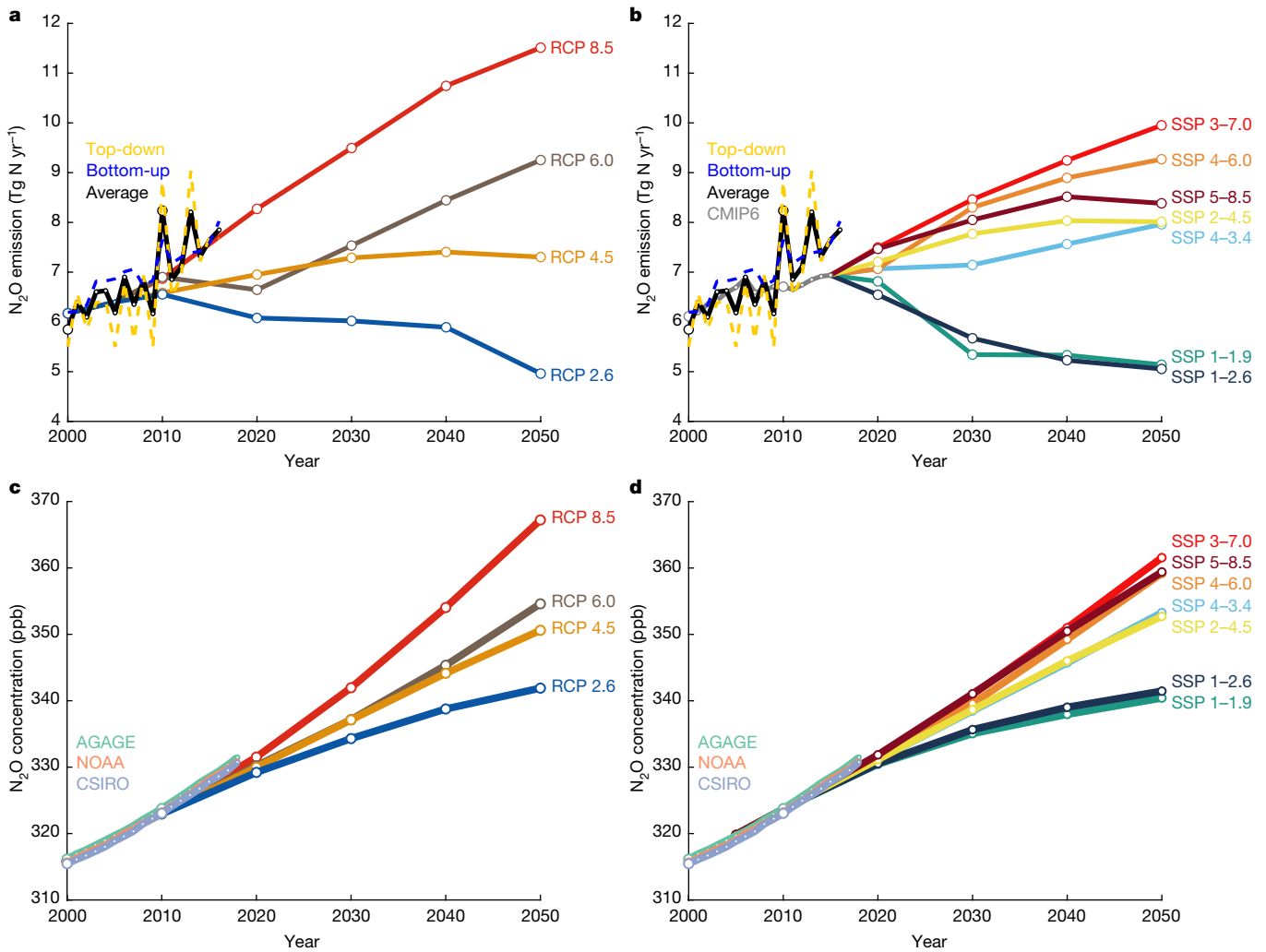
Fig. 4 | Historical and projected global anthropogenic N_2O emissions and concentrations. a–d, Global anthropogenic N_2O emissions (a, b) and concentrations (c, d) compared to the four RCPs in the IPCC assessment report 5 (a, c; ref. 2 ) and the new marker scenarios based on the SSPs used in CMIP6 (b, d; ref. 48 ). The historical emissions data are represented as the mean of the bottom-up and top-down estimates of anthropogenic N_2O emissions, whereas the historical atmospheric concentration data are from the three available
