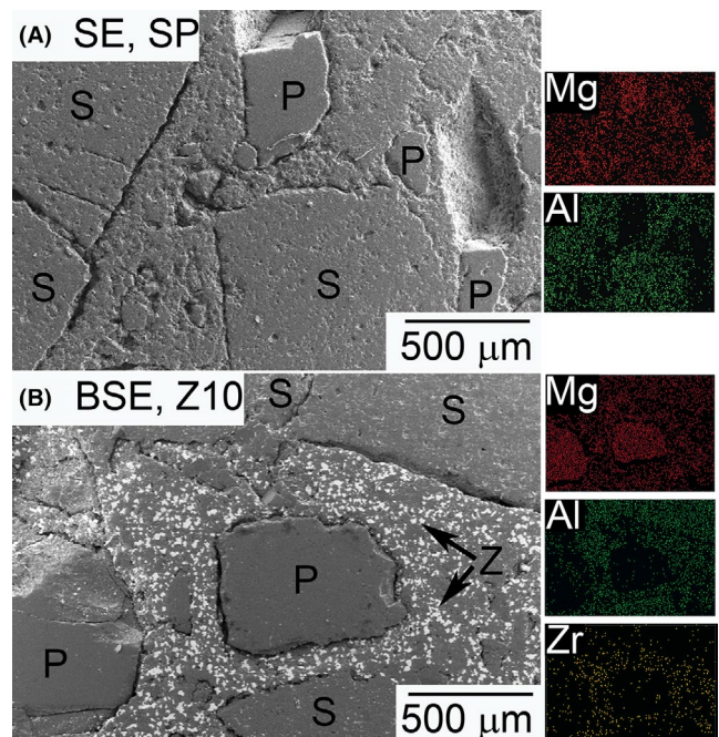
FIGURE 6 A, Secondary electron image of the SP microstructure showing coarse spinel (S) and periclase (P) particles. B, Back scattered electron micrograph of Z10 showing fine white \text{ZrO}_2 (Z) particles in the matrix
