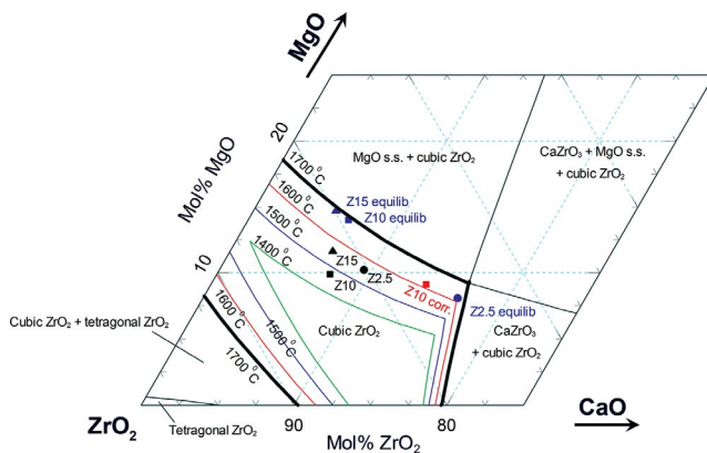
FIGURE 5 Calculated phase diagram of the \text{ZrO}_2 -rich corner of the \text{CaO-MgO-ZrO}_2 system along with boundaries of the cubic \text{ZrO}_2 solid solution at different temperatures. The blue, black, and red markers represent the compositions of the cubic \text{ZrO}_2 phase from equilibrium calculations, and energy dispersive spectroscopy analysis of pristine as well as slag-corroded samples respectively
