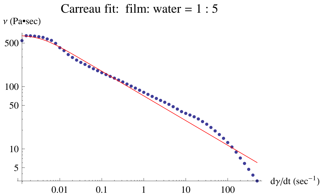
Figure 5.4. log-log plot of viscosity vs. shear rate of a prototype film with swelling ratio: 5. Dots are experimental data, and the solid (red) line is the fitted Carreau model.
