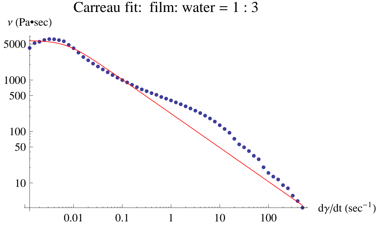
Figure 5.2. The log-log plot of viscosity vs. shear rate of a prototype film with swelling ratio: 3. Dots are experimental data, and the solid (red) line is the fitted Carreau model.
