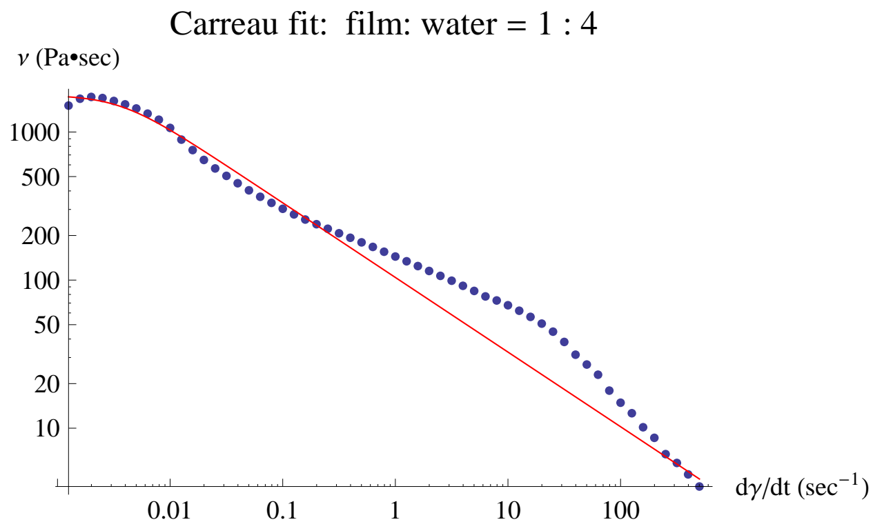
Figure 5.3. The log-log plot of viscosity vs. shear rate of a prototype film with swelling ratio: 4. Dots are experimental data, and the solid (red) line is the fitted Carreau model.
