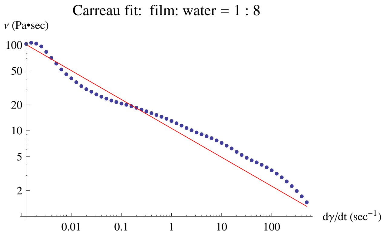
Figure 5.5. The log-log plot of viscosity vs. shear rate of a prototype film with swelling ratio: 8. Dots are experimental data, and the solid (red) line is the fitted Carreau model.
