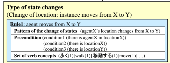
Figure 5: A state-event transformation rule
