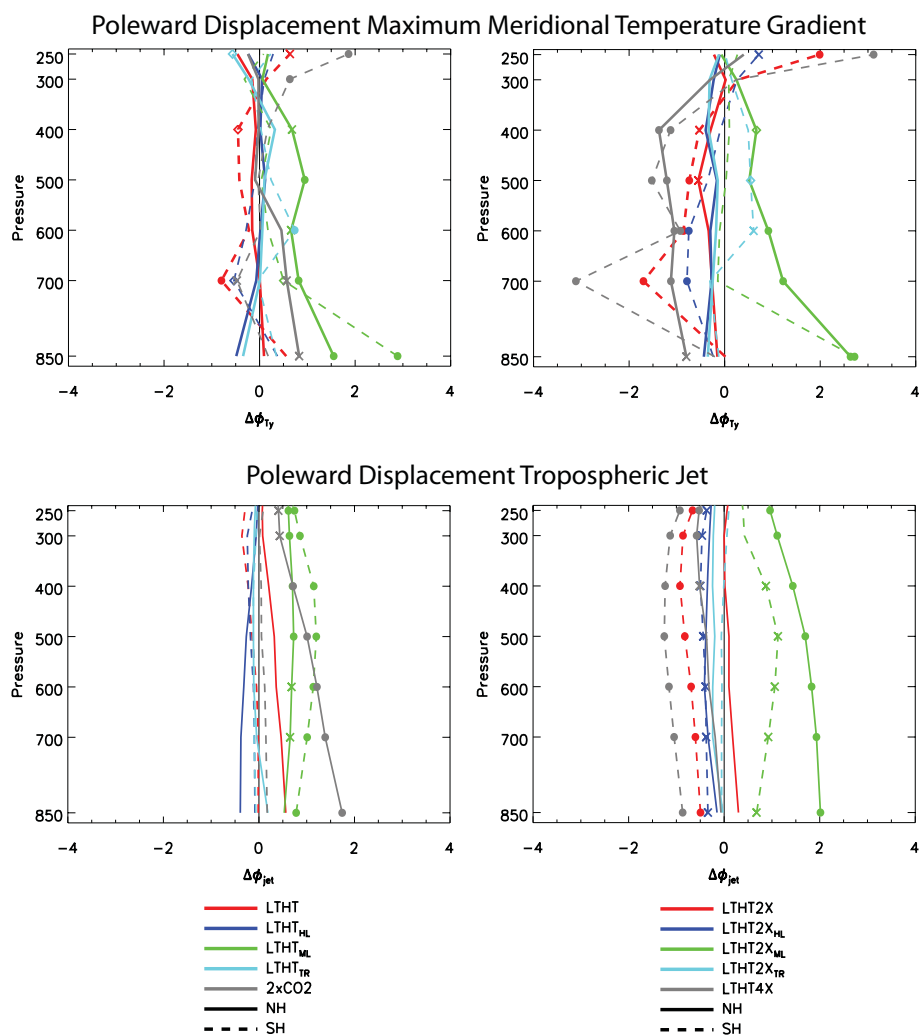
Fig. 4. Poleward displacement of the (top) latitude of the maximum tropospheric temperature gradient ( T_y ) and (bottom) jet for the Northern (solid) and Southern (dashed) Hemisphere for various LTHT and 2\times\text{CO}_2 experiments. Symbols represent significance at the 90 % (diamond); 95 % (cross) and 99 % (dot) confidence level.
