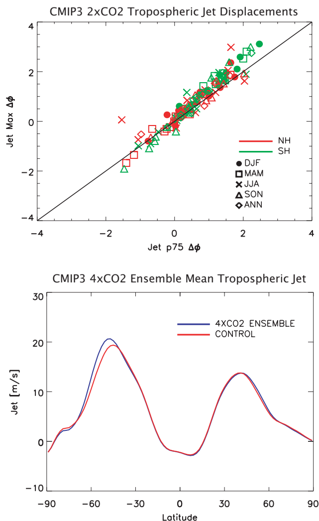
Fig. 1. (Top panel) Tropospheric poleward jet displacement [degrees latitude] based on 12 CMIP3 2×CO 2 equilibrium experiments using the maximum zonal wind method (Jet Max) and the percentile method with the 75th percentile (Jet p75). (Bottom panel) The ensemble annual zonal mean tropospheric jet (850–300 hPa U ) response based on 10 1% to 4×CO 2 transient CMIP3 experiments, along with the corresponding control.
