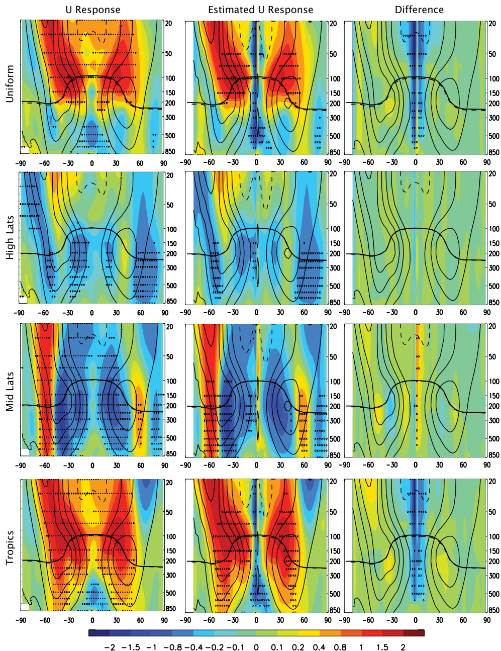
Fig. 5. Zonal annual mean zonal wind response (left), estimated zonal wind response (center) and difference (estimate-actual; right) for the lower-tropospheric heating experiments. The estimated U response is based on thermal wind balance, using the 900 hPa winds as a lower boundary condition. Also shown is the tropopause pressure for the (dashed) control and (solid) experiment. Symbols represent significance at the 90 % (diamond); 95 % (cross) and 99 % (dot) confidence level. Climatological U contour interval is 10 \text{ m s}^{-1} with negative values dashed. Left panels ( U response) are as in Fig. 3.
