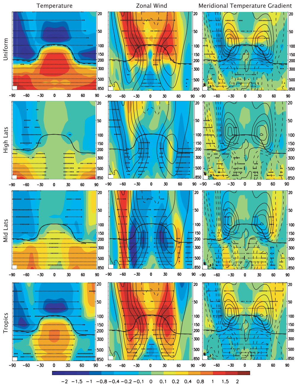
Fig. 3. As in Fig. 2, but based on the lower tropospheric heating (LTHT) experiments.
