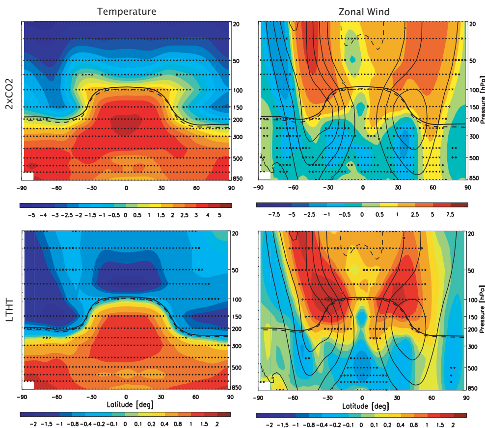
Fig. 7. 2\times\text{CO}_2 (top) and LTHT (bottom) annual mean temperature (left) and zonal wind (right) response. LTHT results, and significance symbols, are as in Fig. 3. Note contour differences between 2\times\text{CO}_2 and LTHT.
