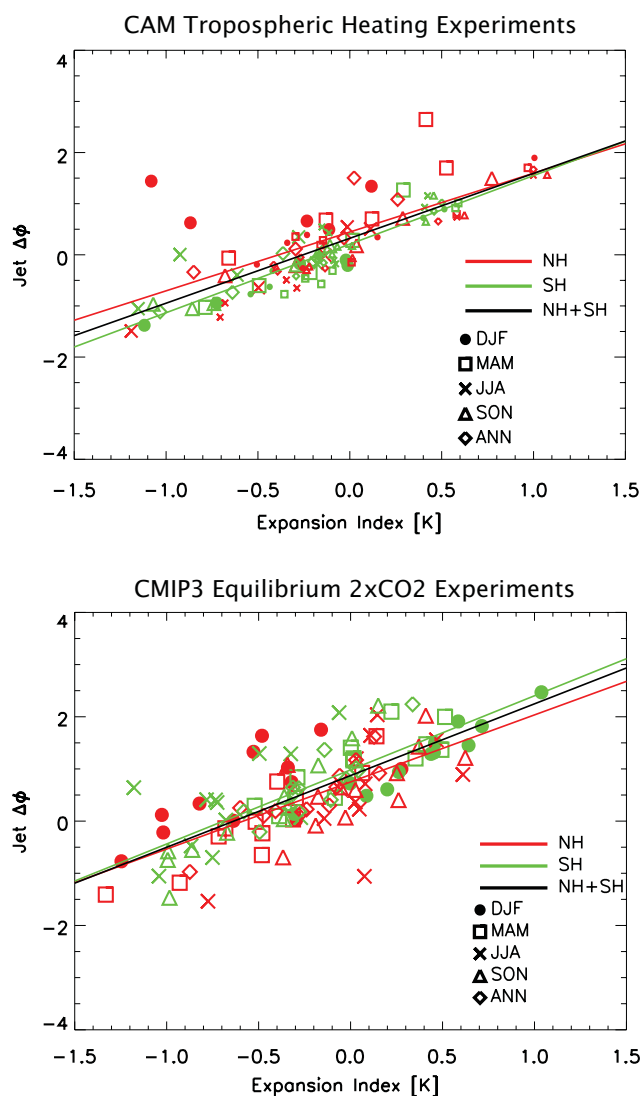
Fig. 10. Scatterplot of tropospheric poleward jet displacement versus the expansion index for the (top panel) CAM tropospheric heating experiments and (bottom panel) 12 CMIP3 2×CO 2 equilibrium experiments. CAM tropospheric heating experiments include the 5 global warming experiments (larger symbols; LTHT, LTHT2 x , LTHT4 x , 2×CO 2 , 8×CO 2 ) and 6 latitude-restricted heating experiments (smaller symbols; LTHT TR , LTHT ML , LTHT HL , LTHT2 xTR , LTHT2 xML , LTHT2 xHL ). Also included are the corresponding linear regression lines, all of which are significant at the 99 % confidence level.
