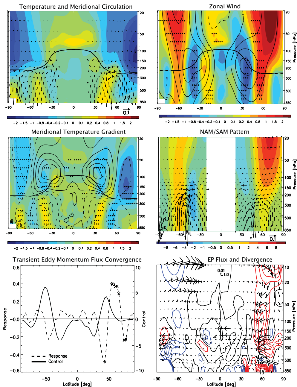
Fig. 9. MAM 10PLO3 HL response of (top left) temperature and meridional circulation, (top right) zonal wind, (middle left) meridional temperature gradient, (middle right) SAM/NAM U pattern, (bottom left) 250 hPa transient eddy momentum flux convergence [ \text{K m s}^{-1} ] and (bottom right) EP flux [ \text{m}^2 \text{s}^{-2} ] and flux divergence [ 10^{-6} \text{ m s}^{-2} ], divided by the standard density. T_y ( U ) contour interval is 2 \times 10^{-3} \text{ K km}^{-1} ( 10 \text{ m s}^{-1} ) with negative values dashed. Units of NAM/SAM are \text{m s}^{-1} per standard deviation of the PC time series. Indicated vector length (top left) represents 0.1 \text{ cm s}^{-1} for the meridional component and -0.1 \times 10^{-4} \text{ Pa s}^{-1} for the vertical component. EP flux divergence contour interval is [-6, -5, -4, -3, -2, -1, 0, 1, 2, 3, 4, 5, 6] , with negative values blue and positive values red. Symbols represent significance as in Fig. 2. Transient eddy momentum flux, \overline{u'v'} is estimated according to \overline{uv} - \bar{u}\bar{v} , where primes denote zonal deviations and overbars indicate zonal averages.
