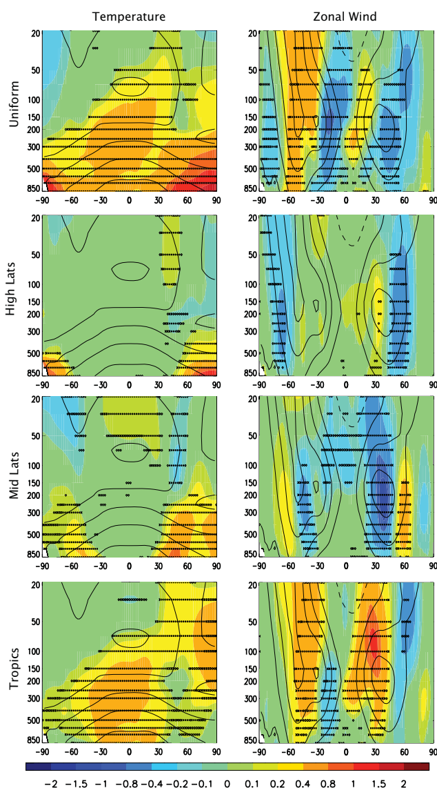
Fig. 6. Zonal annual mean temperature (left) and zonal wind (right) response to heating ( 0.2 \text{ K day}^{-1} ) the lower troposphere using the GFDL AM2.1 model. Symbols represent significance at the 90 % (diamond); 95 % (cross) and 99 % (dot) confidence level. Climatological U contour interval (thin black) with negative values dashed. Climatological T contour interval is 10 \text{ K} .
