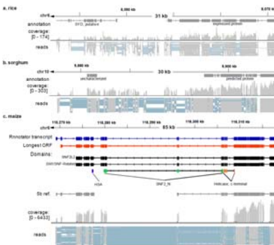
Figure 6. A potential gene fusion, or miss-annotation, in maize when compared to other closely related grass species. Current annotations in rice (a) and sorghum (b) are shown alongside the current maize annotation. In all three grasses this locus is annotated as two separate genes, even though there are reads spanning the gap between the genes in sorghum and maize.
