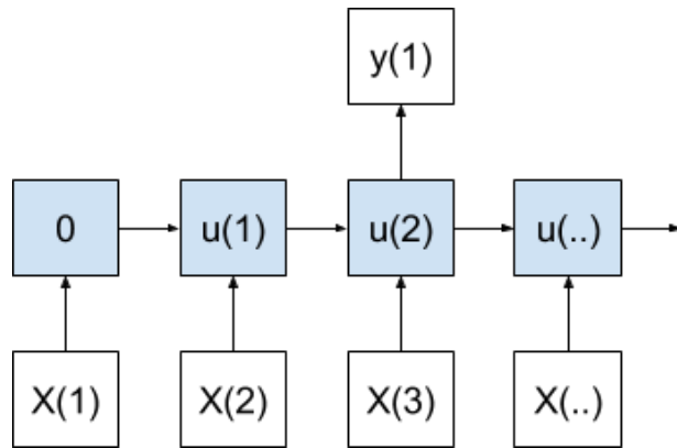
Figure 2.5: Many-to-One Sequence Prediction Model Over Time[Bro17]
