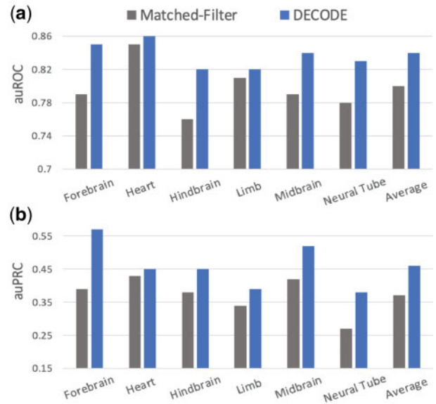
Fig. 4. Benchmarking Against Matched-Filter-Based Model: We benchmarked our trained model against the state-of-the-art model using transgenic mouse enhancers. DECODE produced validation metrics (a, auROC; b, auPRC) that outperformed the state-of-the-art model in all tissue types
