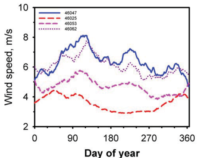
Figure 13. Average wind speeds for selected NOAA buoys.
