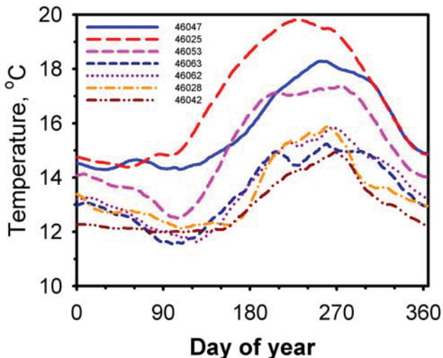
Figure 12. NOAA buoy temperature data.
