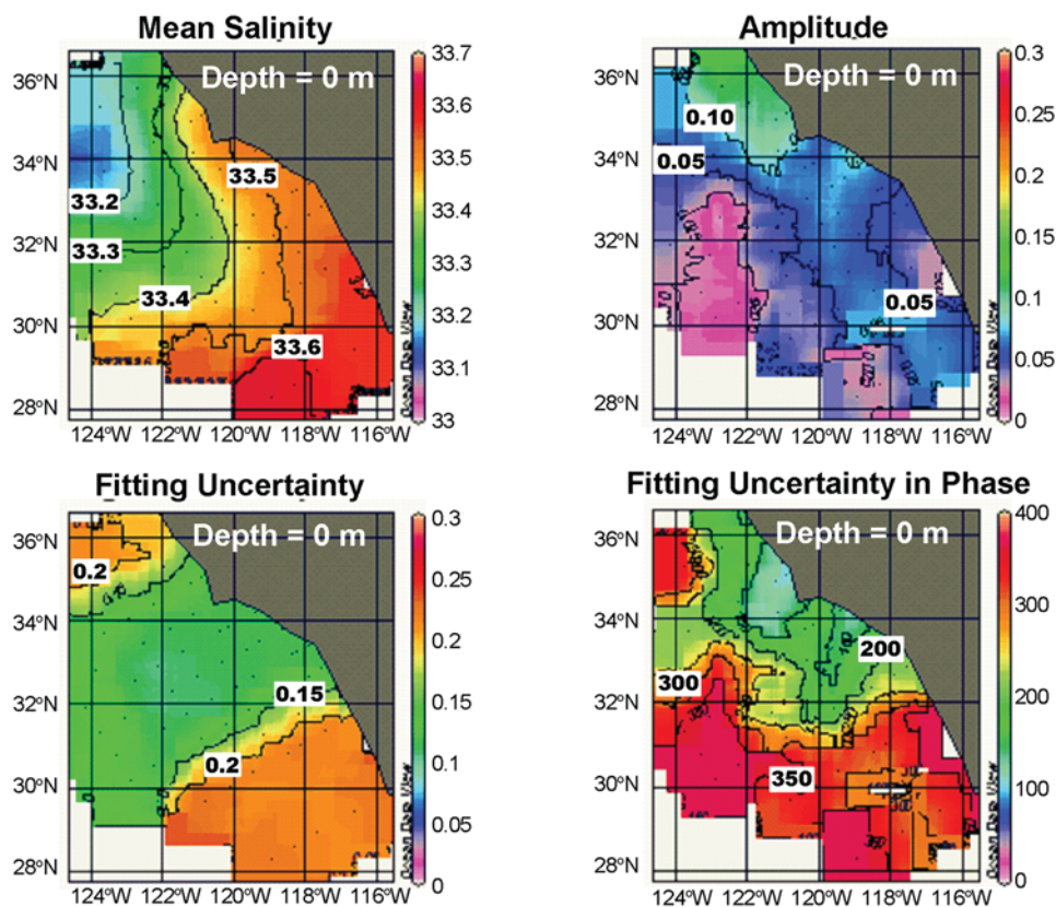
Figure 11. CalCOFI mean salinity (upper left) and fitting uncertainty (lower left). Salinity seasonal amplitude (upper right) and phase uncertainty (lower right) in days.
