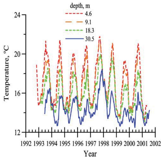
Figure 3. Smoothed CCD data for four depths.
