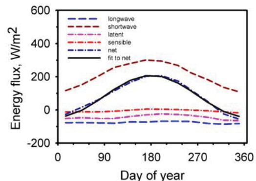
Figure 19. Surface fluxes at Santa Catalina Island from NCEP/NCAR Reanalysis project.
