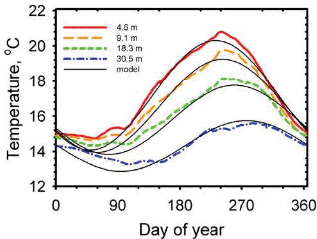
Figure 5. Average temperature for each depth at Santa Catalina and diffusion model with \beta = 0.42 \text{ m}^{-1} and \kappa = 0.00011 \text{ m}^2 \text{ s}^{-1} .
