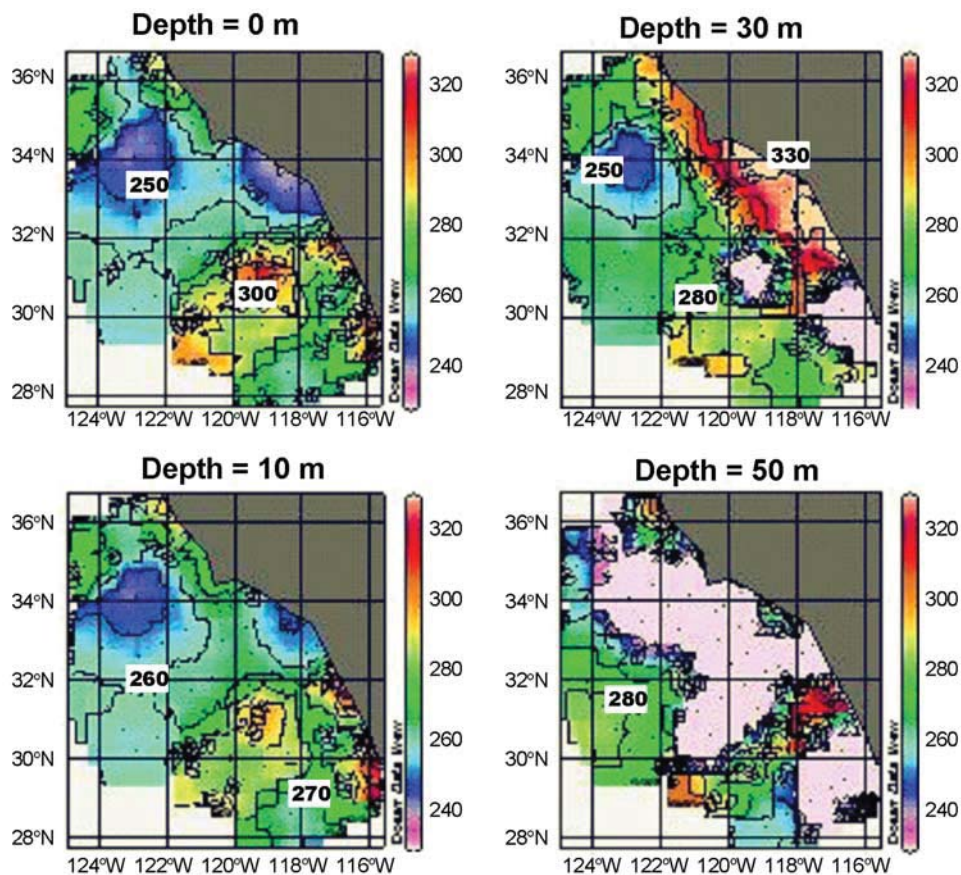
Figure 9. Day-of-year of maximum temperature for CalCOFI data.
