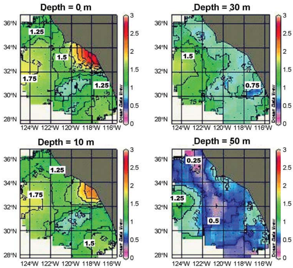
Figure 8. Amplitude of seasonal temperature variations from CalCOFI data.
