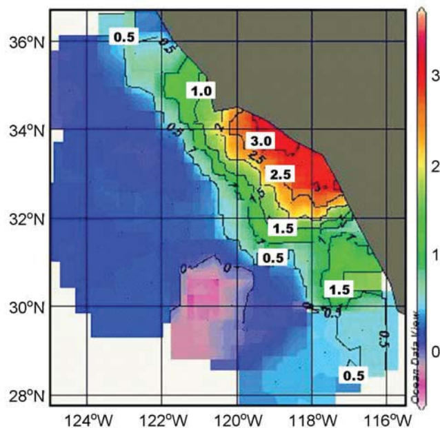
Figure 10. Phase vertical gradient, d/m, from CalCOFI data.
