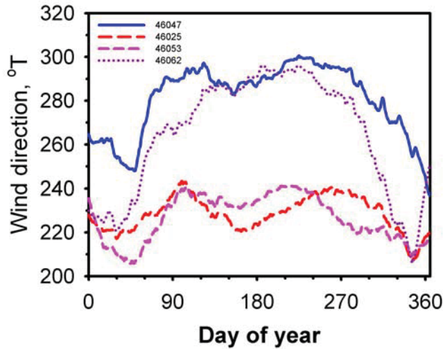
Figure 14. Average wind directions for selected NOAA buoys.
