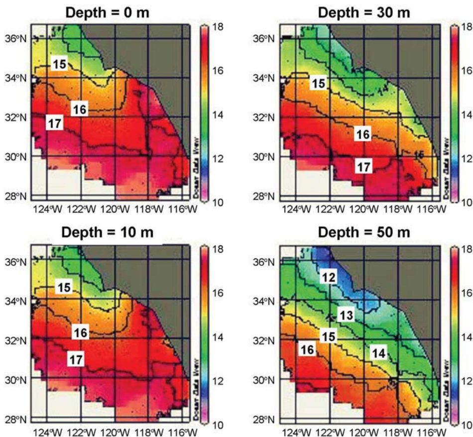
Figure 7. CalCOFI mean temperature at four depths.
