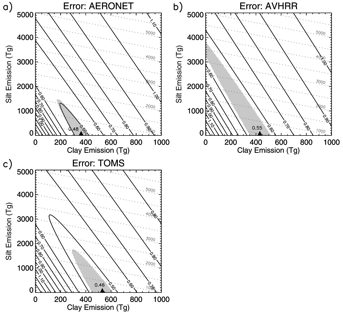
Figure 6. Model error \Phi (solid contours), according to (a) AERONET, (b) AVHRR, and (c) TOMS AOT for the RELEVANT experiment using the GINOX source. The dotted lines mark total emission. The optimal value is marked by the black triangle. The shading indicates values of the error \Phi that are within 5% of the minimum.
