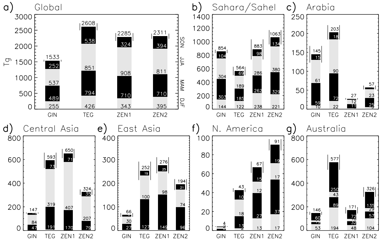
Figure 9. Regional emission of soil dust aerosol (Tg), for the globally optimal RELEVANT solution. The experiments with the GINOX, TEGEN, ZENDER1, and ZENDER2 sources are denoted by GIN, TEG, ZEN1, and ZEN2, respectively. Each bar is divided into seasonal totals for DJF (bottom, light), MAM (above, dark), JJA (above, light), and SON (top, dark). The annual total is given at the top of each bar. The vertical lines bracketing the annual average range between one standard deviation above and below. The Sahara/Sahel average consists of Northern Hemisphere Africa grid boxes. Central Asia is defined between 25–90°E, 32–53°N; and Arabia between 35–60°E (but east of the Red Sea) and 12–36°N.
