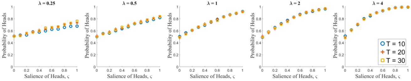
Figure 4: Simulated probability of heads in the simple heads-or-tails coordination game.
