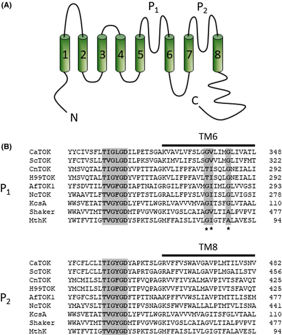
FIGURE 2. Pore region alignment of cloned TOK channels with other known potassium channel subtypes. Alignments were generated using ClustalW 2.0 as per the materials and methods from cloned TOK channels and other potassium channel subtypes of known structure. A, Deduced topology of TOK channel homologues based on hydropathy profile analysis predicting eight putative transmembrane domains flanking two pore-forming domains with intracellular N- and C-termini. B, Sequence alignment of pore regions (P 1 , upper and P 2 , lower) and following transmembrane domain (TM6 or TM8, respectively) of all cloned, functional TOK channels alongside KcsA, Shaker , and MthK. Grey shaded area corresponds to the signature residues of the K + channel selectivity sequence (TXGXGD). (*) indicates location of sites identified in CaTOK and ScTOK that allow inward current
