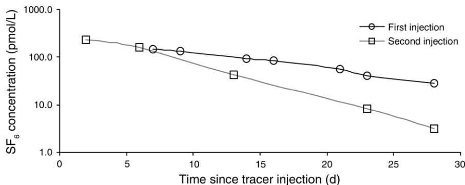
FIG. 18. Concentration of \text{SF}_6 for the two experiments, with both sets of results plotted against time since respective injection (first, 22 June 1998; second, 9 September 1998).
