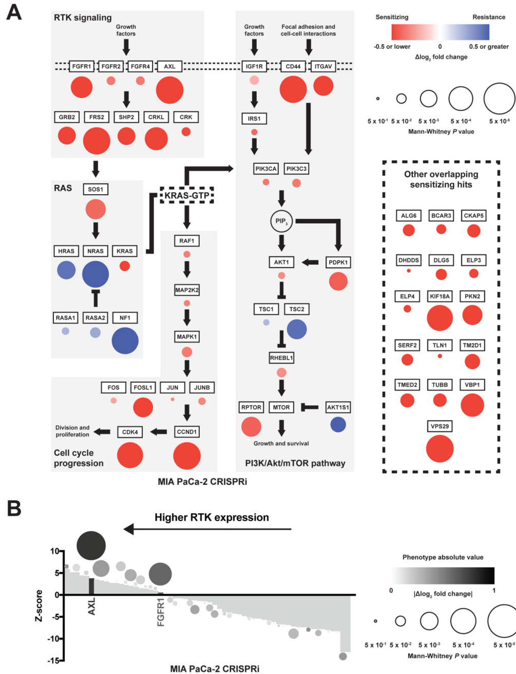
Fig. 3. Critical signaling modules cooperatively sustain a KRAS G12C -driven pro-growth and pro-survival program around KRAS-GTP.
