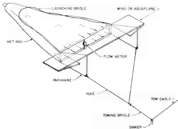
Fig. 1. Manta Net. Schematic diagram
