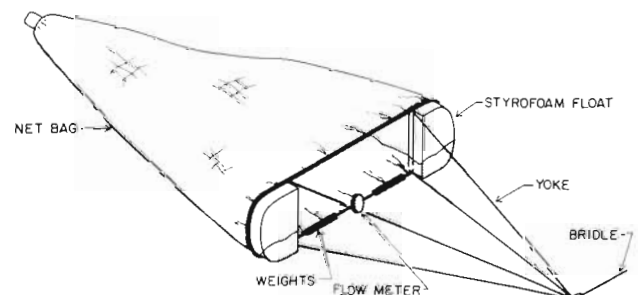
Fig. 3. Neuston Net. Schematic diagram
