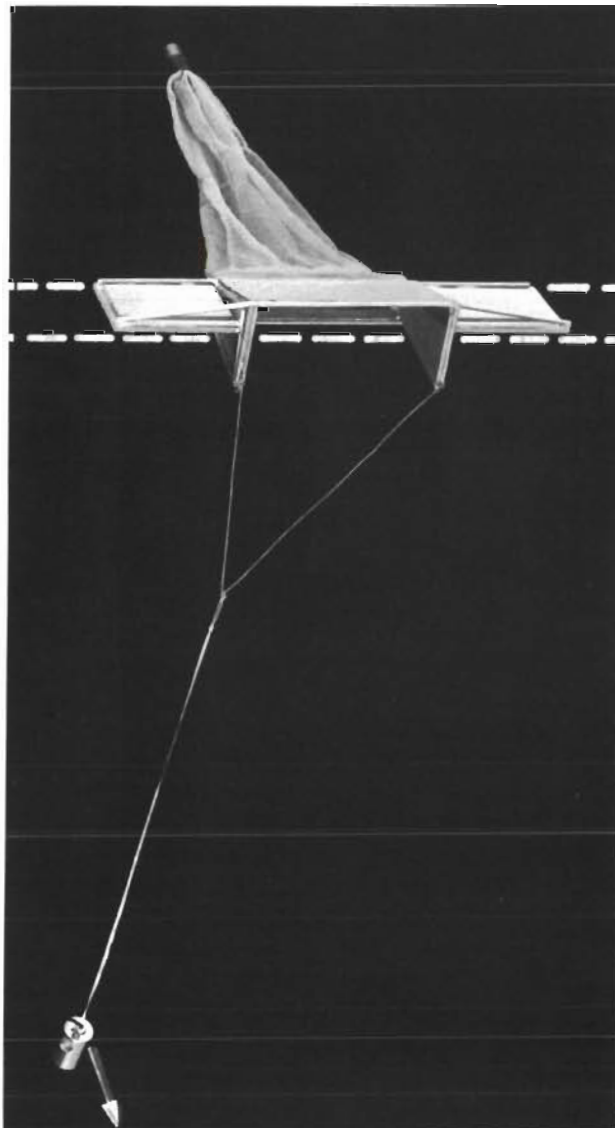
Fig. 2. Manta Net. Scale model. Dashed lines show relative position of sea surface while net is in operation. Arrow: direction of towing
