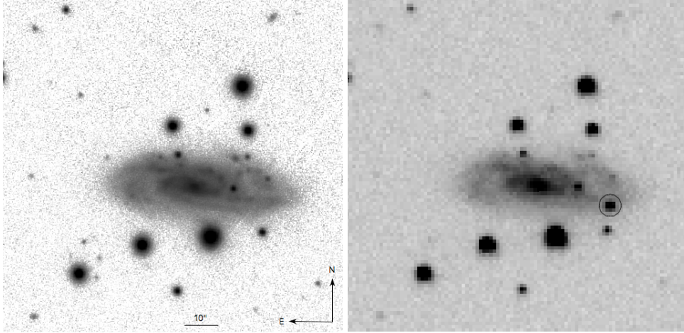
FIG. 1.— Left panel: the PS1 r -band image a of UGC 85, the host galaxy of the supernova SN 2018 fif. Right panel: the P48 r -band image of SN 2018 fif on September 4 2018, at 9:26:50.00 UT. The circle is centered on the SN position.
