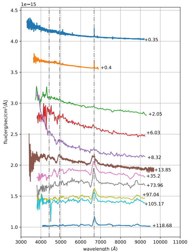
FIG. 3.— The observed spectra of SN 2018fif. An offset was applied for easier visualization. Dashed lines indicate the redshifted emission lines for the Balmer series up to H \gamma . The phase is shown relative to the estimated epoch at which the extrapolated r-band light curve (based on Equation 1) turns to zero: t_0 = 2458351.6537 (2018 August 21), as derived in § 3.1. A color version of this figure is available in the online journal.
