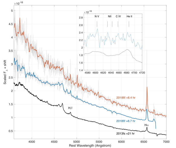
FIG. 7.— Comparison of early spectra of SN 2018 fif (at 8.4 and 8.7 hr) and SN 2013 fs (at 21 hr; from Yaron et al. 2017). SN 2018 fif shows sharp, narrow Balmer lines lacking a broad electron-scattering base. A broad ledge around 4600 Å indicates a likely blend of weak high-ionization lines, suggesting some CSM emission does exist in this event, though less than in SN 2013 fs, see text.
