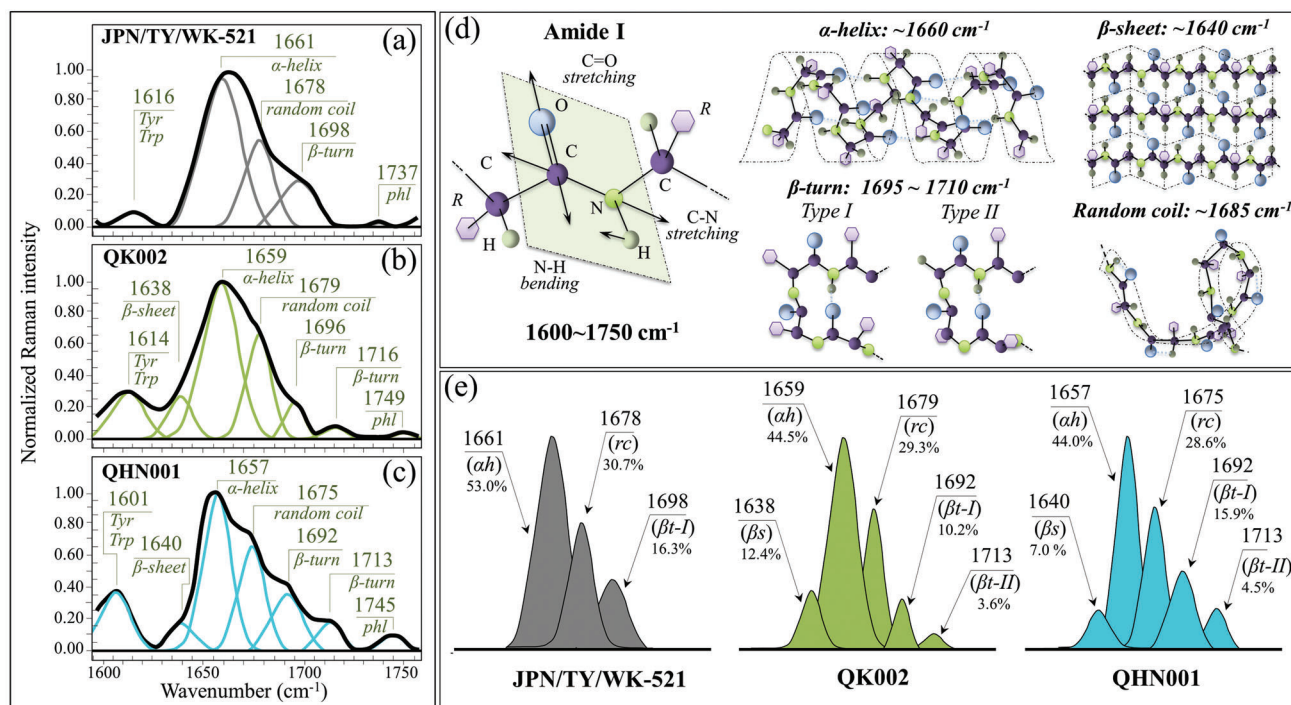
Figure 5. Spectral Zone IV (Amide I, 1600–1750 \text{cm}^{-1} ) of the Raman spectra of a) JPN/TY/WK-521, b) QK002, and c) QHN001 viral strains; spectra are deconvoluted into a sequence of Gaussian-Lorentzian sub-bands (frequencies for selected bands shown in inset). The abbreviations Trp and Tyr refer to tryptophan and tyrosine, respectively. d) Schematic drafts of the Amide I vibrational mode, the different secondary structure of proteins and related frequencies; in e), signals are shown, which are used to estimate the fractions of different protein secondary structures (shown in inset together with the frequencies of the selected signals) found in different strains. The abbreviations \beta s, \alpha h, rc, and \beta -I, \beta -II, and phl represent \beta -sheet, \alpha -helix, random coil, two types of \beta -turn rotamers, and phospholipids, respectively.
