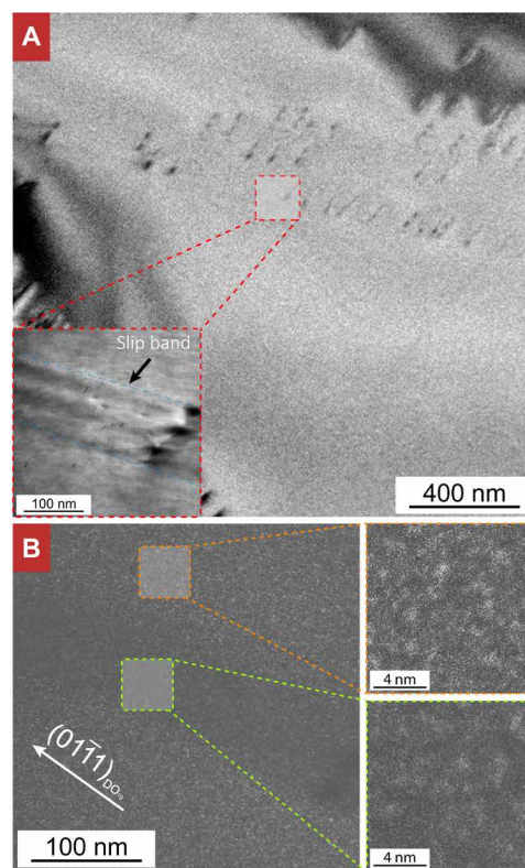
Fig. 4. Energy-filtered DF images of planar dislocation slip bands. (A) Bright-field image showing the relation of a slip band and the imaging area. The slip band is marked and shows weak-fringing contrast in the zoomed-in image. (B) Energy-filtered DF image at the same position of (A) showing the lack of contrast in the slip band.
