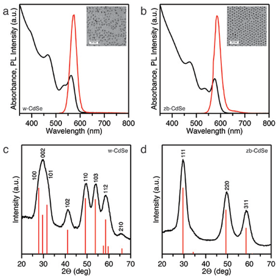
Figure 1. CdSe nanocrystal seeds of wurtzite and zinc-blende crystal structures. (a, b) Absorption (black) and PL (red) spectra with inset of TEM images of wurtzite and zinc-blende CdSe nanocrystals, respectively. (c, d) X-ray diffraction patterns of wurtzite and zinc-blende CdSe nanocrystals with the line patterns of corresponding bulk materials provided for reference. Click here to view larger image.
