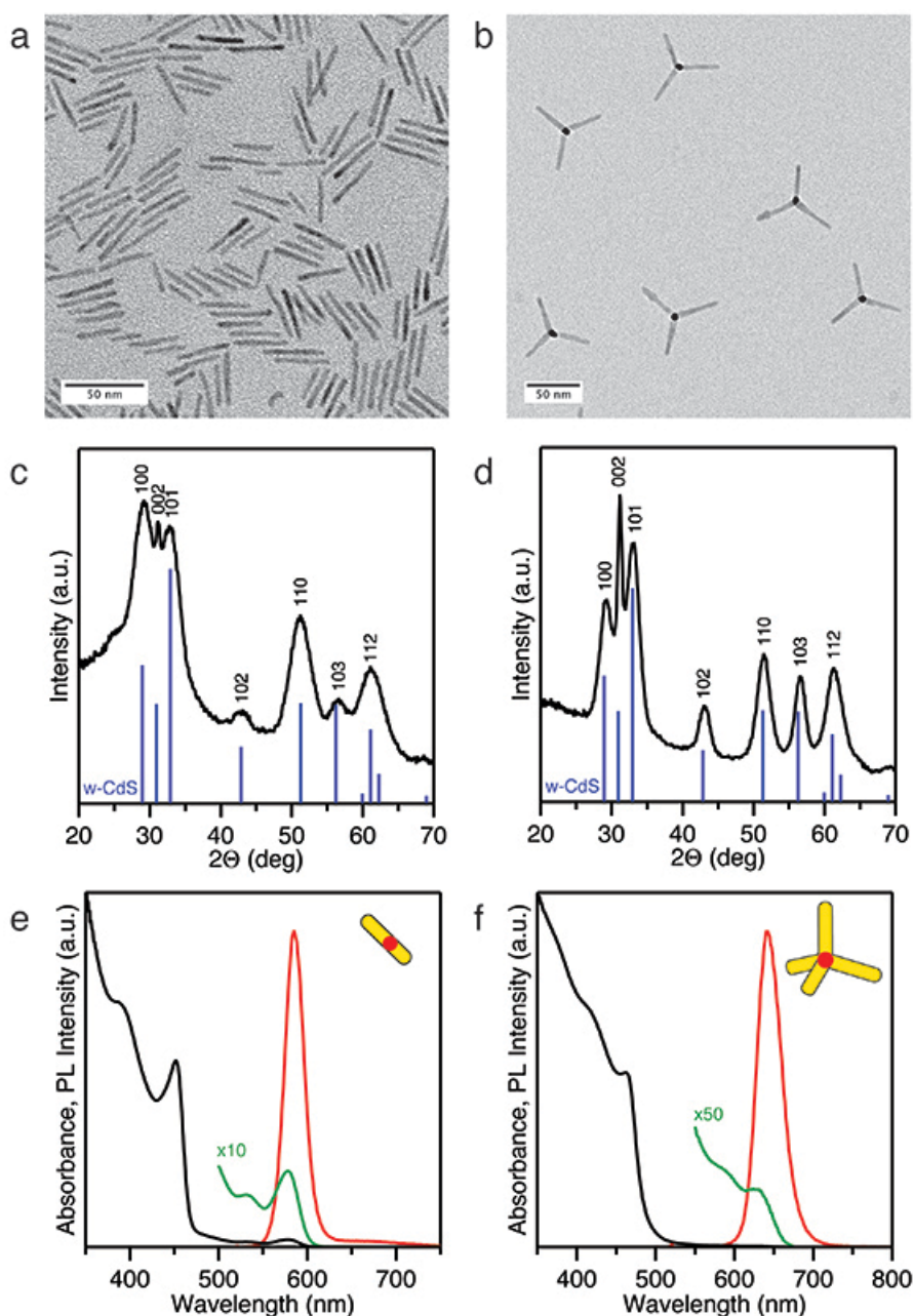
Figure 2. CdSe/CdS seeded heterostructures of rod and tetrapod morphologies. (a, b) TEM images of CdSe/CdS nanorods and CdSe/CdS tetrapods, respectively. (c, d) XRD patterns of CdSe/CdS nanorods and tetrapods. Only reflections from wurtzite CdS are apparent. (e, f) Absorption (black) and PL (red) spectra of CdSe/CdS nanorods and tetrapods. Green line shows magnified absorption spectra to highlight absorption due to the CdSe seed. Click here to view larger image.
