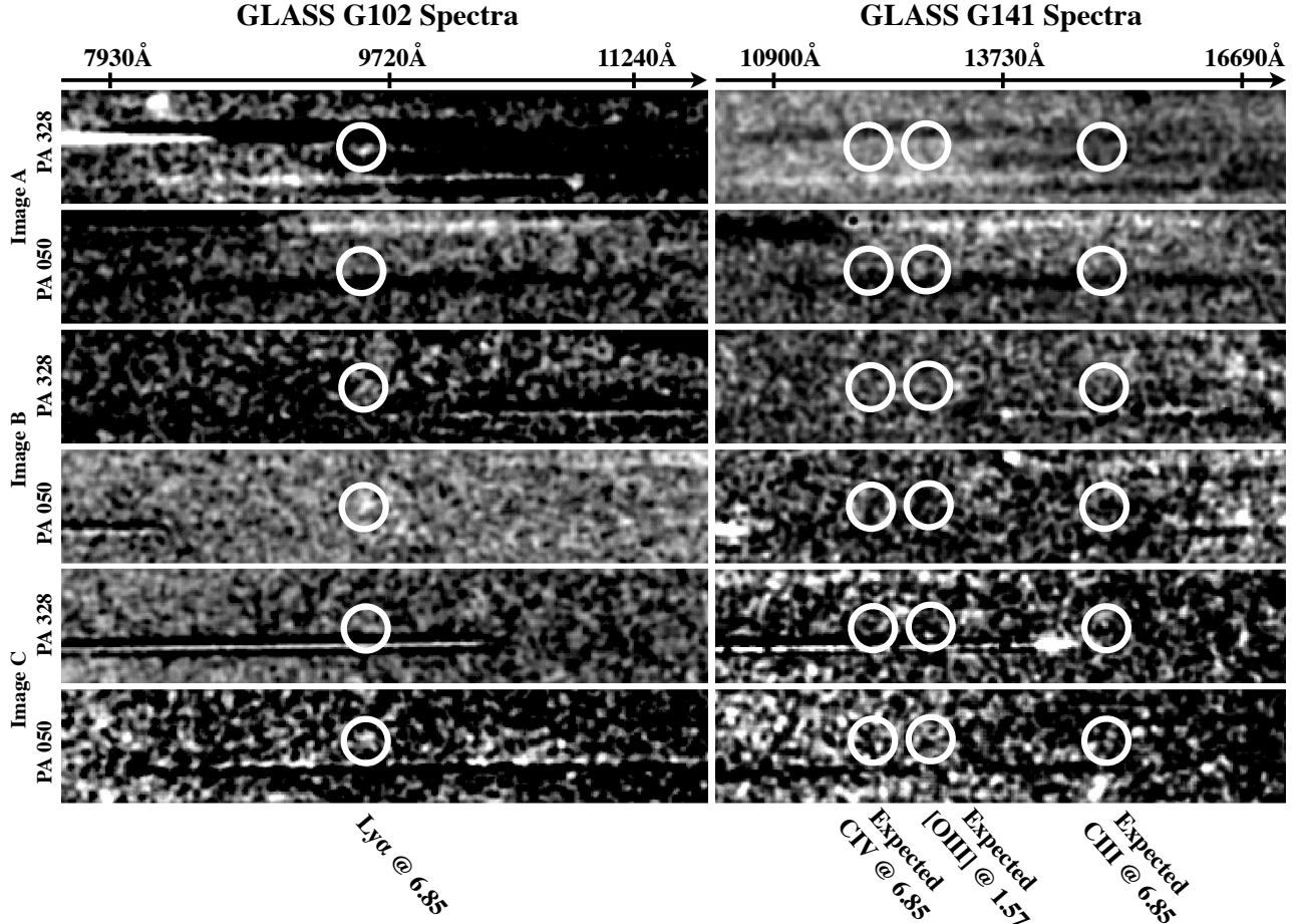
FIG. 3.— Contamination-subtracted HST G102 and G141 grism spectra for Images A, B, and C, obtained as part of the GLASS program. The grism data were taken at two different position angles (PAs; 50^\circ and 328^\circ ), and we show each PA separately. The wavelengths of the observed Ly \alpha and the expected C IV, and C III] lines at z = 6.85 are marked by white circles. We also mark the expected locations of the [O III] line at z = 1.57 . We do not detect any significant flux at the expected wavelength of the potential [O III] line, and the upper limits on [O III]/[O II] strongly support the z = 6.85 Ly \alpha interpretation.
