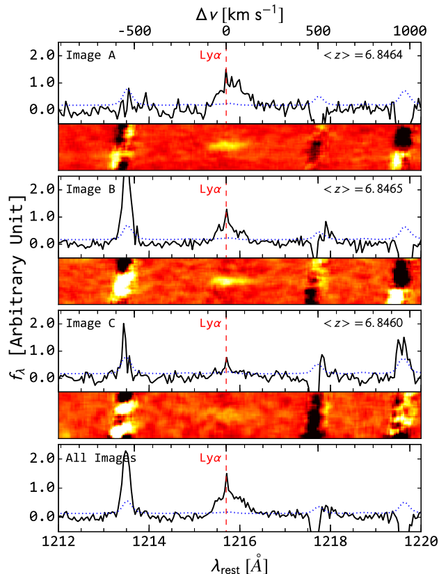
FIG. 2.— Full-depth 1D and 2D Keck/DEIMOS spectra for each image. In the 1D spectra panels, flux density is shown in solid lines, and RMS is shown in dotted lines. The rest-frame wavelength scale is shown on the bottom and the velocity scale is shown on top. The stacked 2D spectra are smoothed by a boxcar filter of width 5 pixels. Spectra are shifted slightly to align the peak wavelengths (shown by a vertical dashed line), and the Ly \alpha redshifts determined by the peaks are indicated in the top-right corners.
