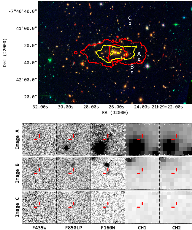
FIG. 1.— Top : RGB image covering the central 3' \times 2' of MACS2129.4–0741 and the locations of Images A, B, and C. The critical curve ( \mu = 100 ) of the cluster at z = 6.85 ( z = 1.57 ) is shown as red (yellow) lines. The z = 1.57 critical curve does not come close to reproducing the parity of the triple images. Bottom : Cutouts ( 5'' on each side) of all three images in F435W, F850LP, F160W, IRAC ch1, and IRAC ch2 (from left to right) are shown in each row. There is a nominal 3.3\sigma detection in the F850LP data for Image A that we consider spurious based on its morphology, and we exclude the F850LP magnitude of Image A in our analysis.
