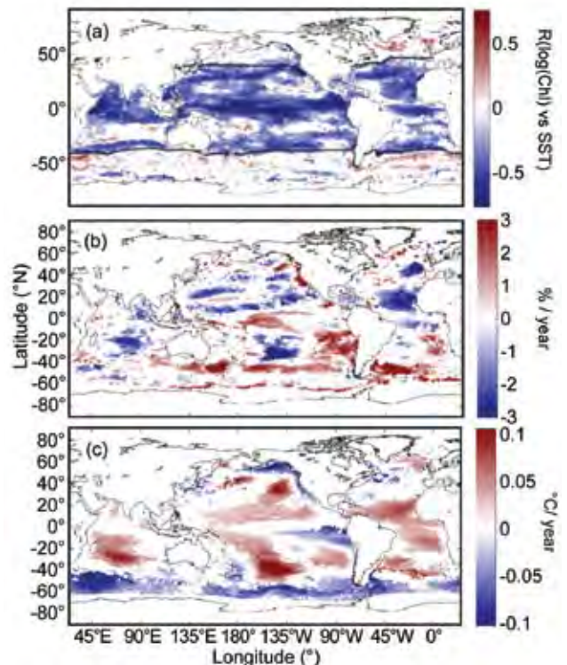
FIG. 3.38. (a) Spatial distribution of the local-scale correlation coefficient ( R ) between \ln(\text{Chl}) and SST, (b) local-scale time trends in \ln(\text{Chl}) anomalies (in \% \text{ yr}^{-1} ), and (c) local-scale time trends in SST anomalies (in ^\circ\text{C yr}^{-1} ). Only significant (95% confidence interval) correlations and trends are plotted. Calculations are made over the entire SeaWiFS record (Oct 1997–Dec 2010) and on a local-scale 1^\circ bin in latitude and longitude. Also shown in (a) is the 15^\circ\text{C} SST isotherm (black line).
