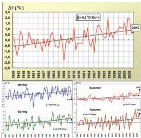
FIG. 7.38. Anomalies of average annual and seasonal air temperatures averaged over the Russian territory for the period 1939–2010 (1961–90 base period).
