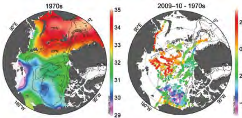
FIG. 5.6. Anomalies of salinity at 20 m depth in 2009–10 (right) relative to 1970s climatology (left). The 500 m and 2500 m isobaths have been plotted using the IBCAO grid.
