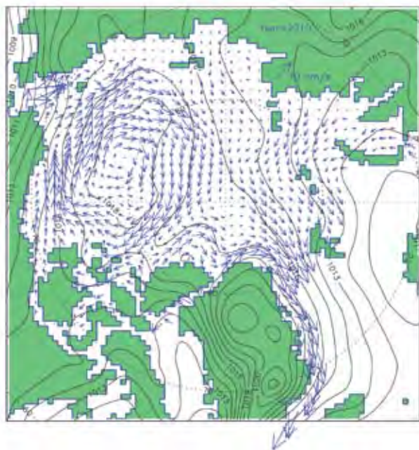
FIG. 5.4. Annual 2010 simulated wind-driven ice motion (arrows) and sea level atmospheric pressure (hPa, black lines). Results are from a 2-D coupled ice-ocean model (Proshutinsky and Johnson 1997, 2011) forced by wind stresses derived from 2010 NCEP/NCAR re-analysis six-hourly sea level pressure fields.
