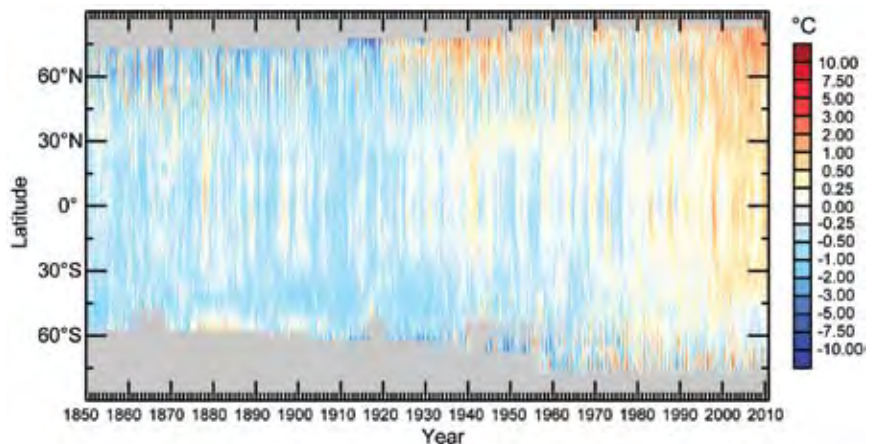
FIG. 2.4. HadCRUT3 monthly mean anomalies of surface temperature by latitude based on the 1961–90 base period. Gray areas indicate regions where data are unavailable.
