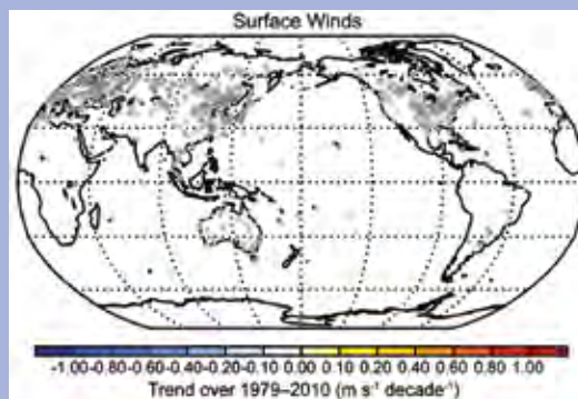
FIG. 2.45. Observed trends in wind speeds at locations with long and fairly homogeneous data records.
