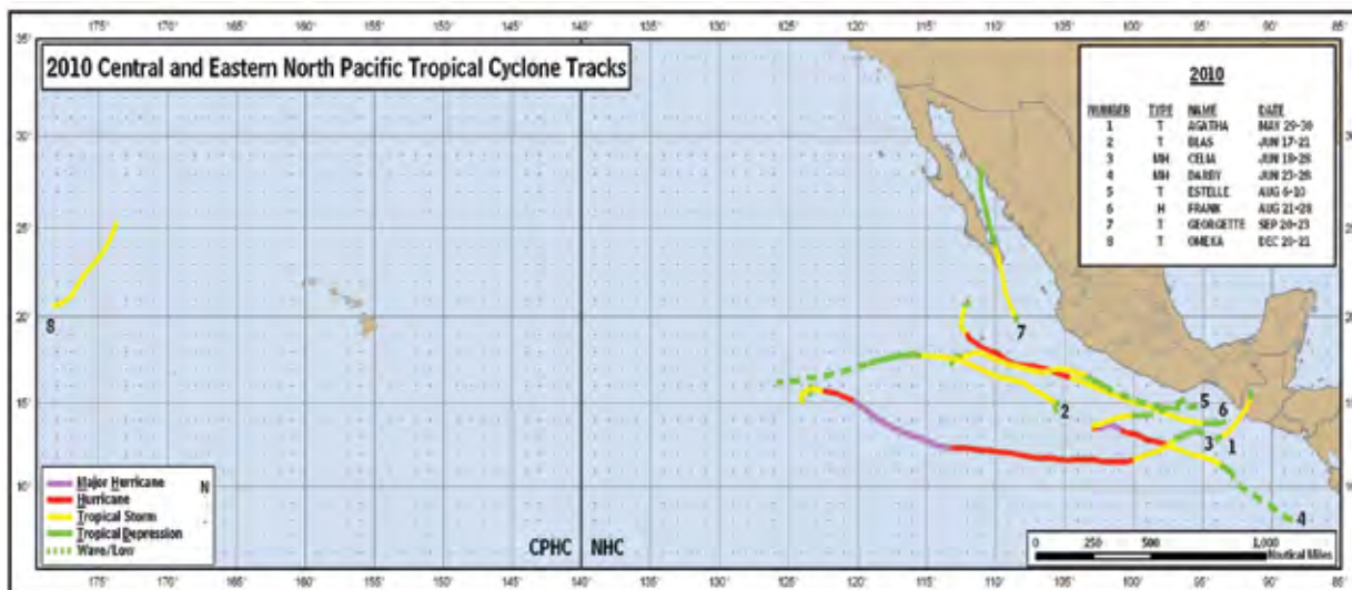
FIG. 4.19. Storm track map for the Eastern Pacific hurricane basins, including all tropical cyclones that occurred in the Eastern North Pacific and Central North Pacific basins [Source: NOAA's National Hurricane Center (NHC) and Central Pacific Hurricane Center (CPHC)]. Tracks are color coded by intensity (wave/low, tropical depression, tropical storm, hurricane, and major hurricane). Also shown is the delineation of the forecast area of responsibility at 140°W between NOAA's NHC and CPHC.
