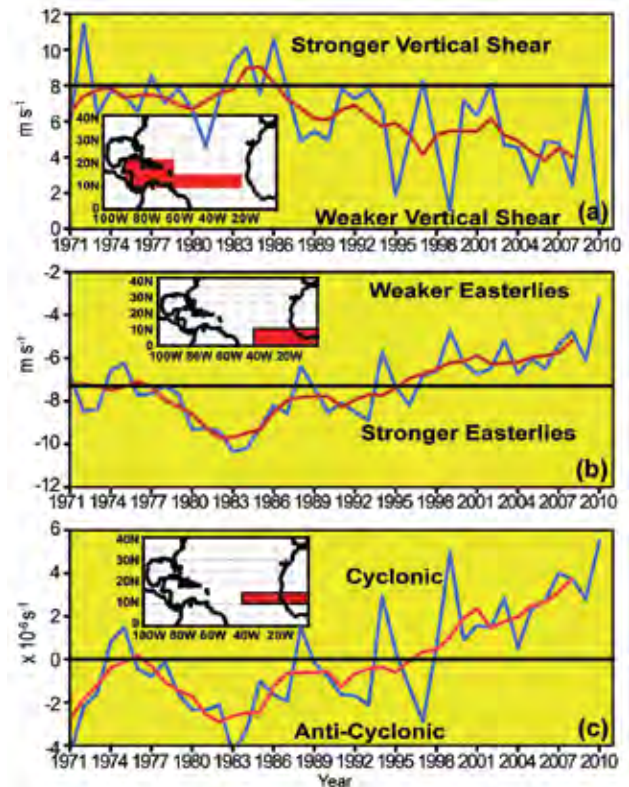
FIG. 4.18. Time series showing consecutive August–October values of area-averaged (a) 200 hPa–850 hPa vertical shear of the zonal wind ( \text{m s}^{-1} ), (b) 700-hPa zonal wind ( \text{m s}^{-1} ), and (c) 700-hPa relative vorticity ( \times 10^{-6} \text{ s}^{-1} ). Blue curve shows unsmoothed values and red curve shows a five-point running mean of the time series. Averaging regions are shown in the insets.
