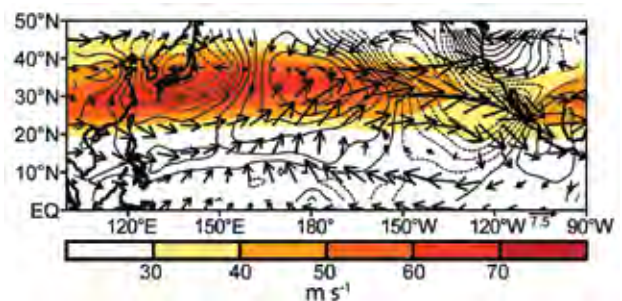
FIG. 4.6. DJF 2009/10: Total 200-hPa wind speed ( \text{m s}^{-1} , shaded), anomalous wind vector, and anomalous horizontal wind speed tendency ( d/dt ) (contours, interval is 1 \times 10^{-4} \text{ m s}^{-2} ). Solid (dashed) contours show anomalous speed acceleration (deceleration), where
