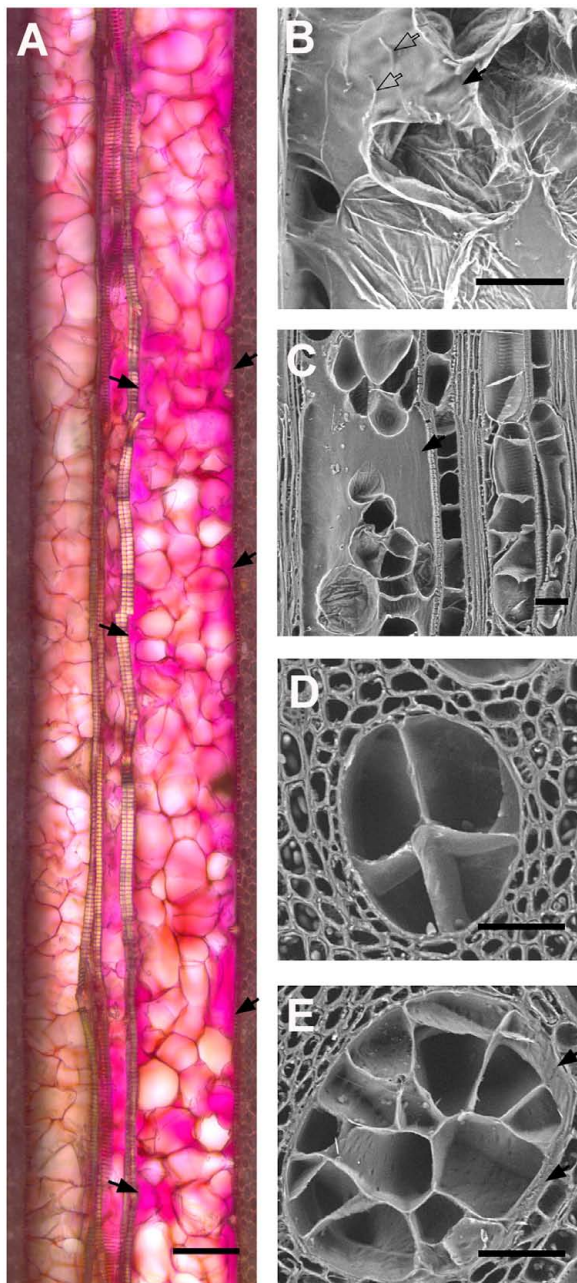
FIGURE 5 | Effect of vessel diameter on the quality of vessel occlusion with tyloses in four V. vinifera L. cultivars. (A) Micrograph of longitudinal section of occluded vessels found in Phaeomonniella chlamydospora inoculated grape cv Cabernet Sauvignon (bright field, ruthenium red). Note the difference in the diameter of the vessel on the left side (about 90 \mu\text{m} of diameter) and the vessel on the right side (about 150 \mu\text{m} of diameter). Note the compact network of tyloses that walls off the narrowest vessel while large pockets of gels (solid black arrows) are present in the wider vessel. (B,C) Scanning electron micrograph of a longitudinal section of P. chlamydospora infected grapevine cv Thompson Seedless. Note the presence of a large pocket of gels observed in occluded vessel. (D,E) Scanning electron micrographs of occluded vessels of various diameters as observed in the stem of grapevine cv Thompson Seedless infected with P. chlamydospora . Note the increasing number of tyloses occluding cross-sectional area of vessels with the increase of vessel diameter. (A,B) Scale bar = 100 \mu\text{m} . (C–E) Scale bar = 50 \mu\text{m} .
