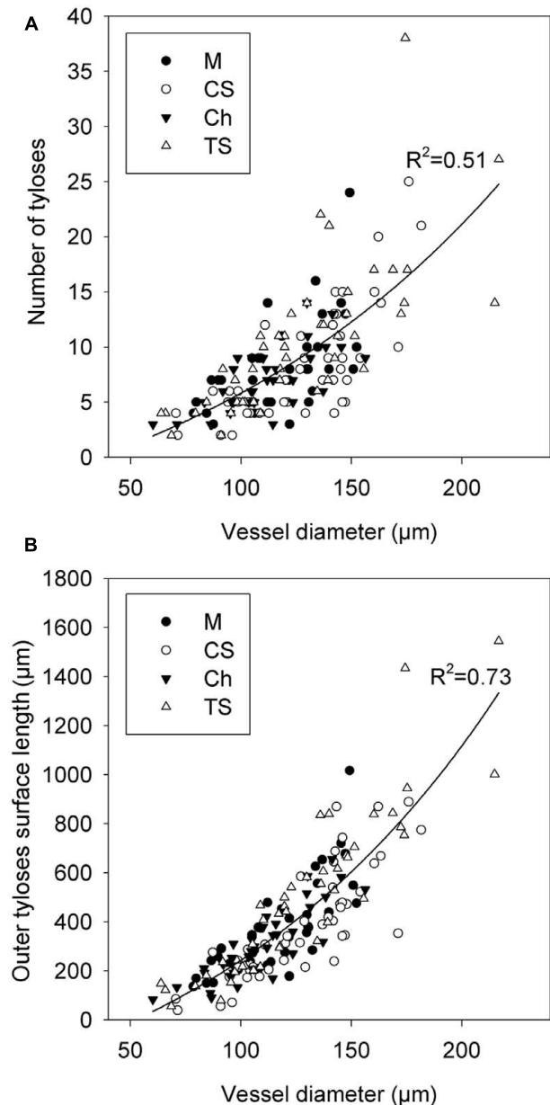
FIGURE 6 | Modeling of the effect of xylem vessel diameter on the quality of vessel occlusion with tyloses across four V. vinifera L. cultivars. (A) Graphic showing the relation between the arithmetic diameter of vessel and the number of tyloses occluding the cross-sectional area of vessel. (B) Graphic showing the relation between the arithmetic diameter of vessel and the outer tyloses surface length (OTSL). Regression curve in (A,B) represent the general model developed with data collected from the grapevine cvs Merlot (M), Chardonnay (Ch), Cabernet Sauvignon (CS), and Thompson Seedless (TS).
