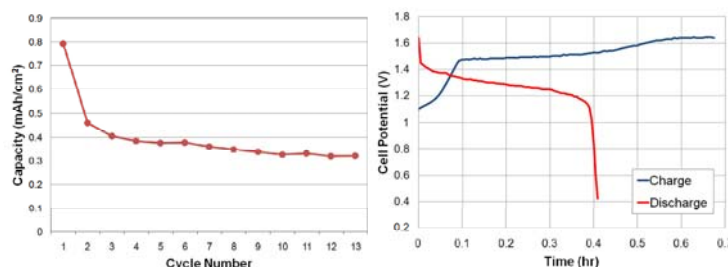
Discharge capacity during cycling of the zinc-silver cell with PVA – KOH – H 2 O alkaline solid polymer electrolyte
