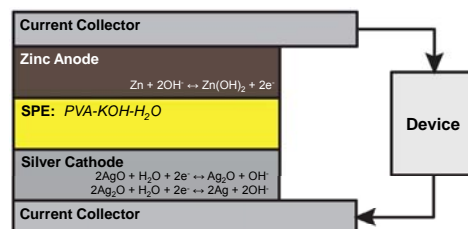
Schematic of zinc-silver battery system with charge-discharge reactions
