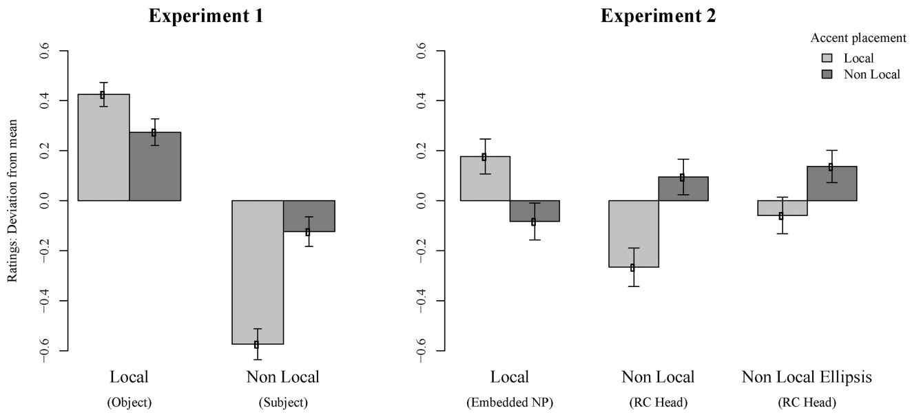
Figure 3. Ratings for each condition expressed as deviations from the grand mean for Experiments 1 and 2.
