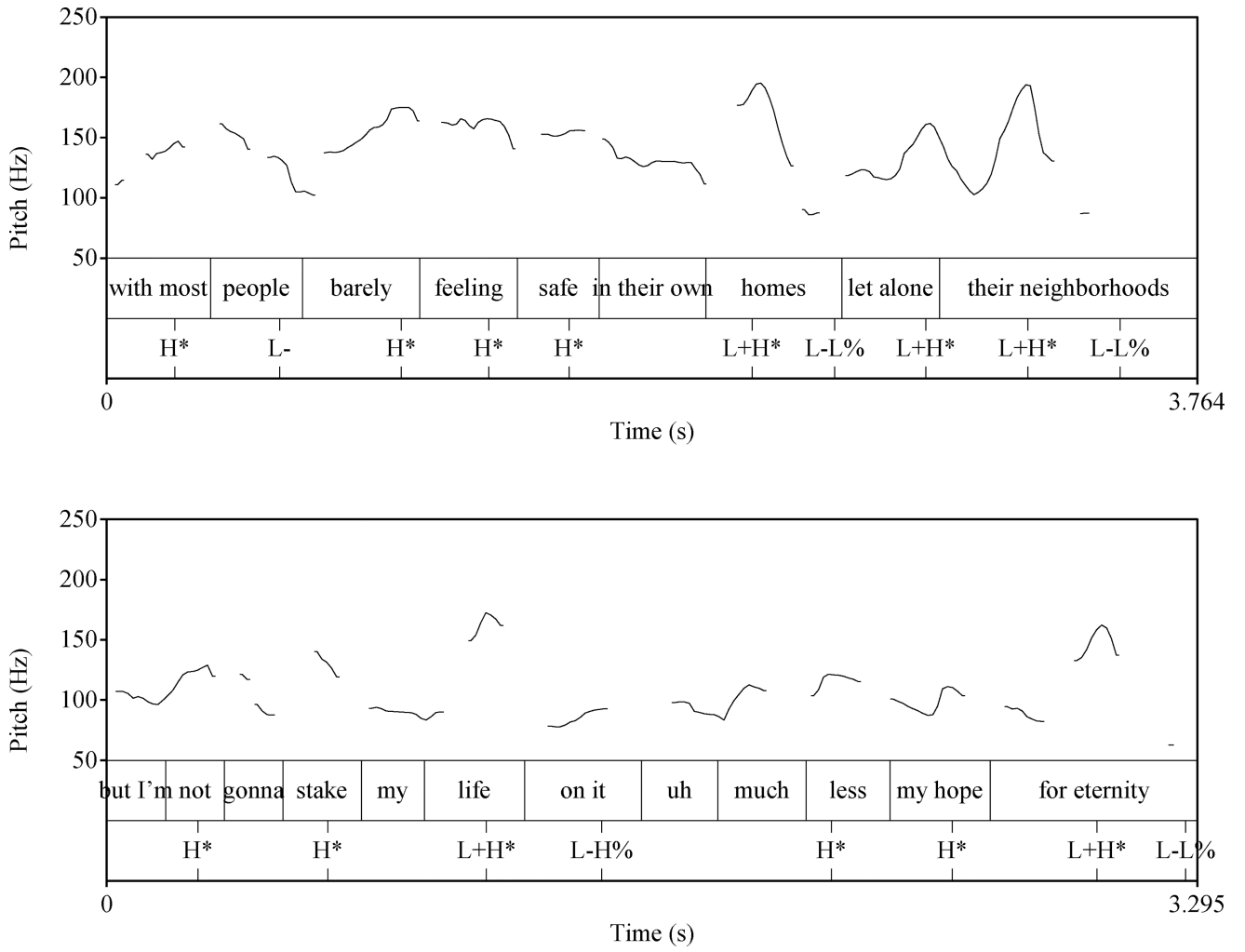
Figure 1. Pitch track of examples with a local correlate (a) and a non-local correlate (b).
