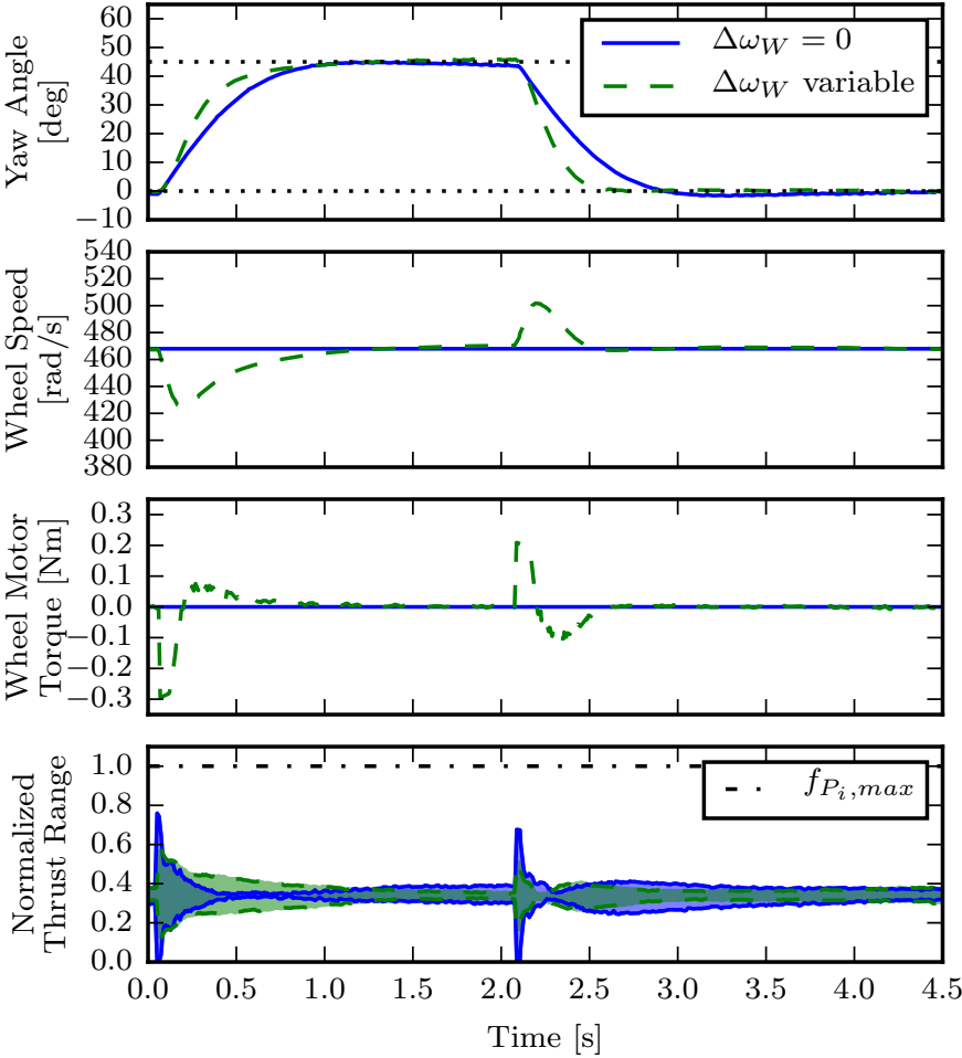
Figure 3.8: Response of the large vehicle to a step change in desired yaw of 45° followed by a second step change in desired yaw back to 0°. A controller that allows for some error in the desired momentum wheel speed outperforms a controller that does not allow the wheel to accelerate or decelerate.
