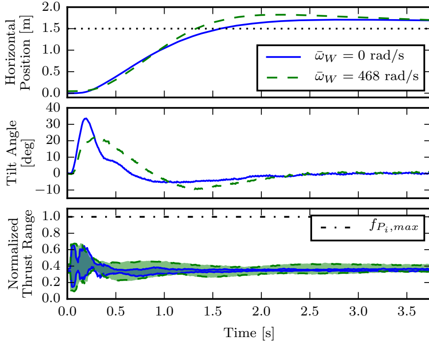
Figure 3.9: Responses of the large vehicle to a 1.5 m horizontal step change in desired position both with and without the momentum wheel spinning. The vehicle with the wheel spinning requires slightly more time to reach the desired position.
