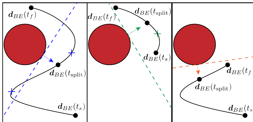
Figure 5.1: A graphical depiction of Algorithm 1. Three sequential calls to CHECKSECTION (as defined in Algorithm 1) are shown. The red circle represents the convex obstacle and the solid black line represents the trajectory in time. In the first call to CHECKSECTION (shown in the left panel), two critical points (drawn as crosses) of the distance to the separating plane (drawn as a dashed line) are found. The trajectory is found to cross the separating plane between t_f and the critical points occurring after t_{split} , prompting a recursive call to CHECKSECTION . As shown in the middle panel, this sub-trajectory is found to not collide with the obstacle because it lies entirely on the opposite side of the newly computed separating plane. Next, the original trajectory (left) is again found to cross the separating plane between t_s and t_{split} , leading to a second recursive call to CHECKSECTION . As shown in the right panel, this sub-trajectory is also found to lie entirely on the opposite side of the newly computed separating plane, proving that the entire trajectory does not collide with the obstacle.
