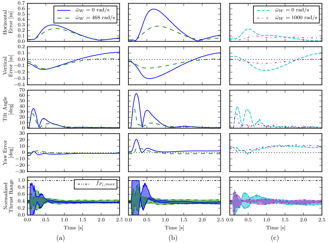
Figure 3.6: Responses to a torque impulse caused by a collision with a mass dropped from above. The tilt angle is defined as the angle between z_B^E and the vertical, and the normalized thrust range is defined as the minimum range that contains all four thrust forces, which are normalized to the maximum thrust f_{\max} . The response of the larger vehicle to a 0.092 \text{ N m s} torque impulse is shown in (a), the response of the larger vehicle to a 0.186 \text{ N m s} torque impulse is shown in (b), and the response of the smaller vehicle to a 4.7 \times 10^{-4} \text{ N m s} torque impulse is shown in (c). The performance of the vehicle is improved in all three cases when the wheel is spinning, and an even more significant improvement is observed when the motor forces saturate, as shown in (b).
