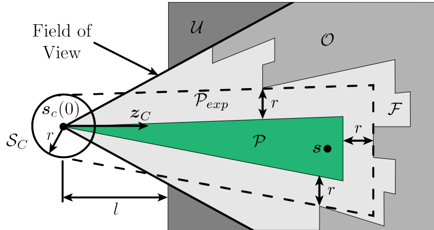
Figure 6.1: 2D side view illustrating the generation of a single pyramid \mathcal{P} , shown in green, from a single depth image and given point s . The depth values of each pixel are used to define the division between free space \mathcal{F} and occupied space \mathcal{O} . Because the depth camera has a limited field of view, we additionally consider any space outside the field of view farther than distance l from the camera to be unknown space \mathcal{U} , which is treated the same as occupied space. The expanded pyramid \mathcal{P}_{exp} (dash-dotted line) is first generated such that it does not contain any portion of \mathcal{O} or \mathcal{U} , and then used to define pyramid \mathcal{P} such that it is distance r from any obstacles.
